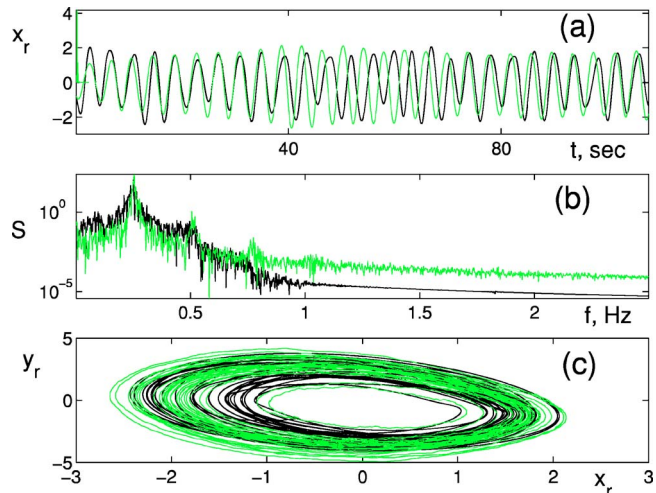
FIG. 4. (Color online) (a) Time series of the respiratory oscillations x_r(t_n)=s_r(t_n) in arbitrary units (black line) obtained from measurements of central venous blood pressure. The sampling rate was 90 Hz after resampling of the original signal. Inferred time series of the respiratory oscillator is shown by the green line. (b) Power spectra of the respiratory oscillations obtained, respectively, from the real data (black line) and from the inferred oscillations (green line). (c) Limit cycles of the respiratory oscillations x_r(n),y_r(n) obtained from real data as described in the text (black line) and from the inferred oscillations (green line).
