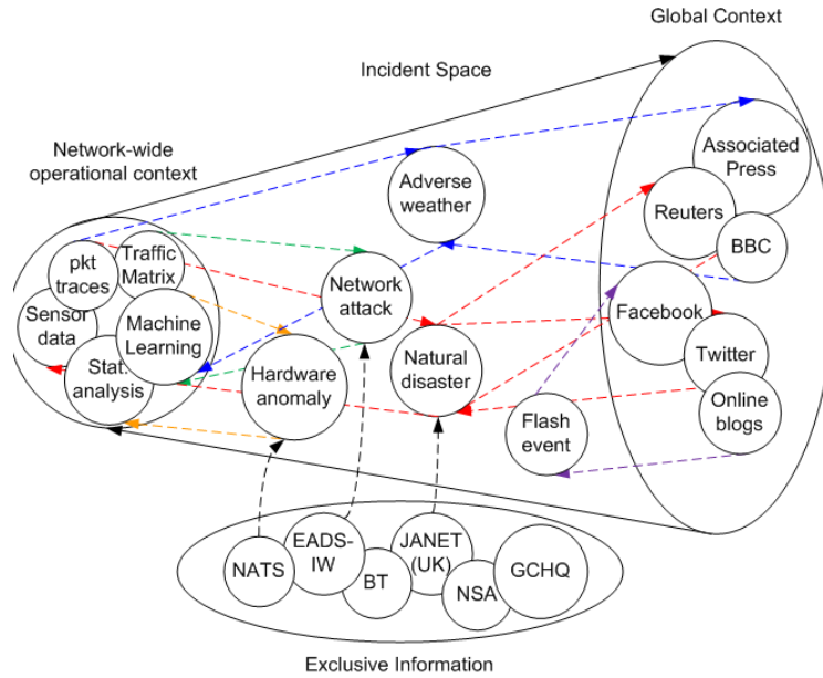
Fig. 1. The SAI^2 Framework
