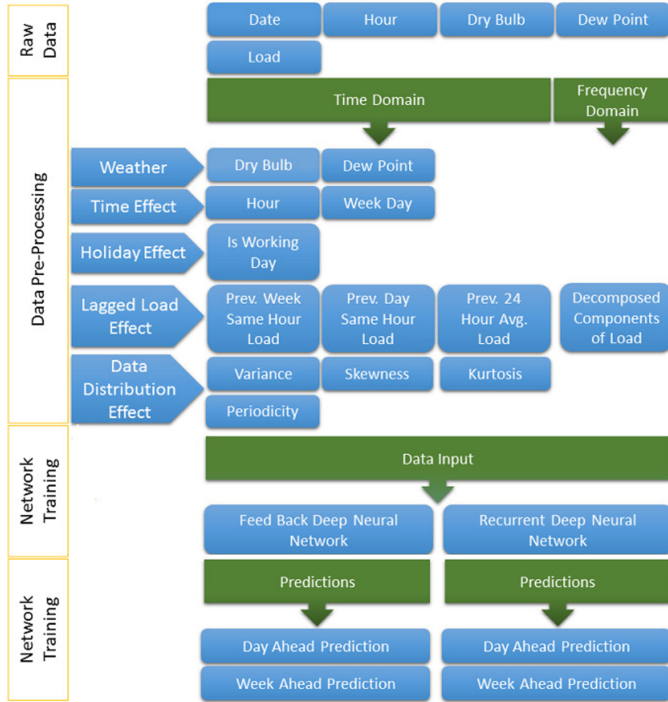
Fig. 3. Visual Description of Load Prediction Methodology
