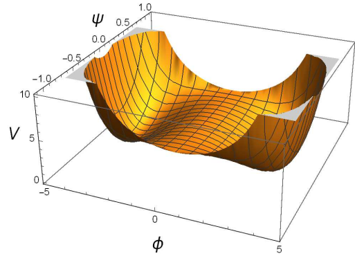
Fig. 1: The potential given by Eq. (2.5).
