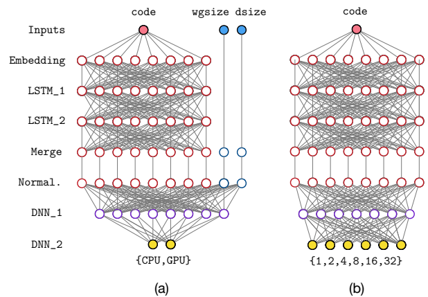
Figure 4: DeepTune neural networks, configured for (a) heterogeneous mapping, and (b) thread coarsening factor. The design stays almost the same regardless of the optimization problem. The only changes are the extra input for (a) and the number of nodes in the output layer.
