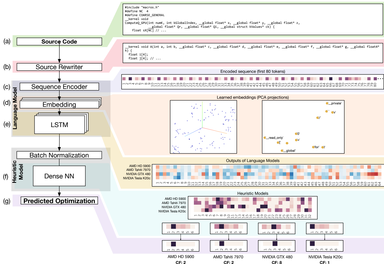
Figure 9: Visualizing the internal state of DeepTune when predicting coarsening factor for Parboil’s mtx10 benchmark on four different architectures. The activations in each layer of the four models increasingly diverge the lower down the network.
