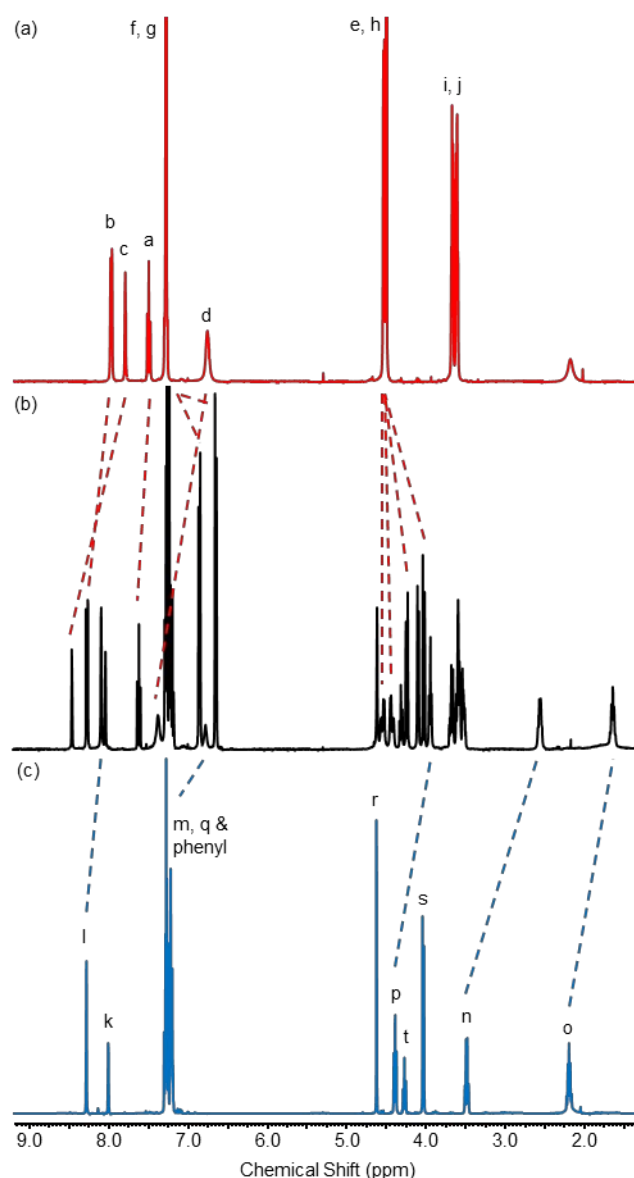
Figure 2: 1 H NMR spectra of (a) macrocycle 1 , (b) rotaxane 6 and (c) axle 8 (CDCl 3 , 400 MHz, 298 K). For atom labels see Schemes 1 and 2.
