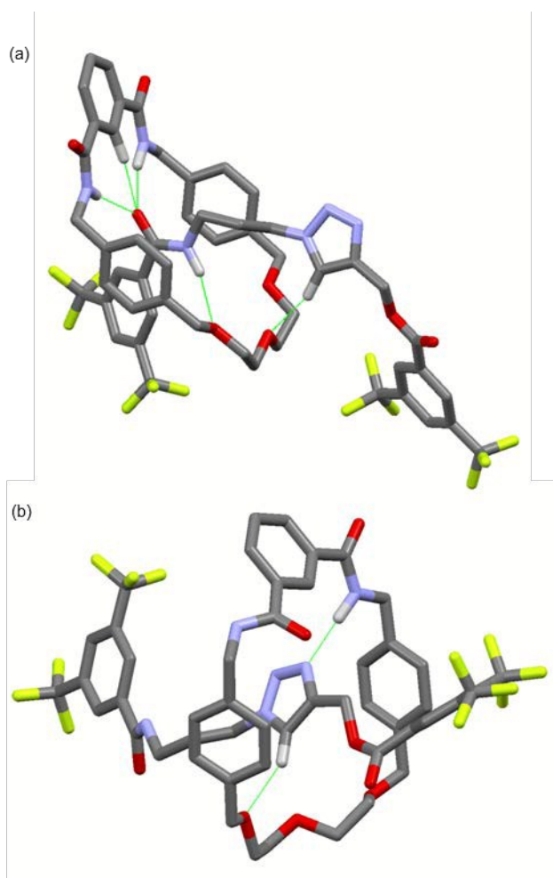
Figure 3: Minimum energy structures of rotaxane 7 with macrocycle occupying (a) amide and (b) triazole "stations". Hydrogen bonds are represented by green dashed lines. Hydrogen atoms not participating in hydrogen bonding are omitted for clarity.
