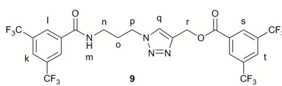
Scheme 2: Syntheses of rotaxanes 6 and 7 and non-interlocked axles 8 and 9 . Reaction conditions: (i) cat. \text{Cu}(\text{CH}_3\text{CN})_4\text{BF}_4 , cat. TBTA, DIPEA, \text{CH}_2\text{Cl}_2 .
