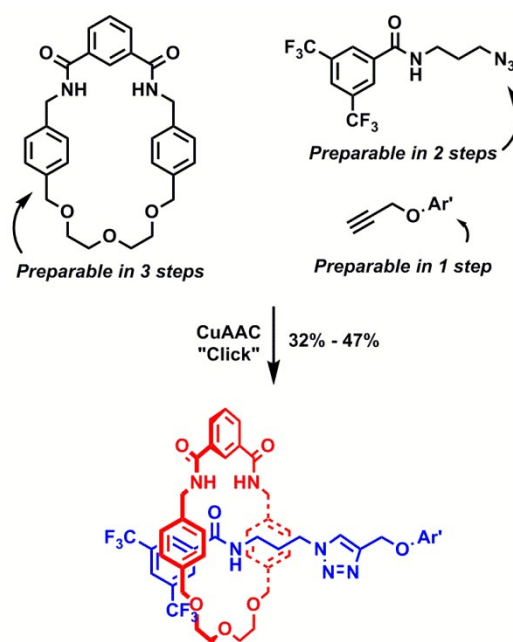
Figure 1: Schematic representation of the rapid synthesis of rotaxanes utilizing a single amide hydrogen bond templating motif and the CuAAC click reaction.
