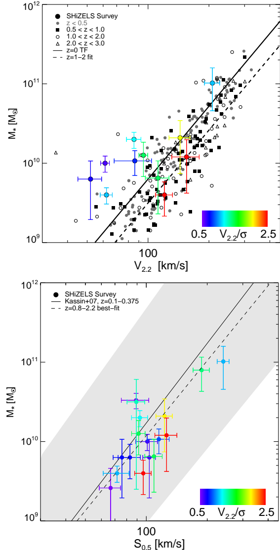
Figure 5. Top: Evolution of the stellar mass TF relation measured from the SHiZELS survey at z = 0.8 - 2.23 colour-coded using the V_{2.2}/\sigma ratio. We only show our galaxies consistent with rotating systems together with their 1\sigma velocity and stellar mass uncertainties. The solid line denotes the TFR at z = 0 from Pizagno et al. (2005). The dashed line represent the best-fit TF relation at z = 1 - 2 from Swinbank et al. (2012a) based on the compilation of high-redshift points from Miller et al. (2011, 2012 z = 0.6 - 1.3 ); Swinbank et al. (2006 z = 1 ); Swinbank et al. (2012a z = 1.5 ); Jones et al. (2010b z = 2 ); Cresci et al. (2009 z = 2 ) and Gnerucci et al. (2011b z = 3 ). Galaxies with lower relative rotational support tend to be scattered to lower values along the velocity axis. This is consistent with the result found by Tiley et al. (2016). Bottom: The M_*-S_{0.5} relationship measured from the SHiZELS survey at z = 0.8 - 2.23 . The error bars show the 1\sigma stellar mass and S_{0.5} mass uncertainties. The data is colour-coded as in the image above. The solid line represents the relation at z \sim 0.2 from Kassin et al. (2007) and the shaded area represents its 1\sigma uncertainty. The dashed line corresponds to the best-linear-fit to our data. Our scatter is tighter than the intrinsic M_*-S_{0.5} scatter. The slope ( 0.32 \pm 0.2 ) and the intercept at 10^{10} M_{\odot} ( 1.98 \pm 0.09 ) found from our best-fit are consistent with the uncertainties of the z \sim 0.2 relation. This is consistent with no evolution of the M_*-S_{0.5} relation with redshift up to z = 2.23 .
