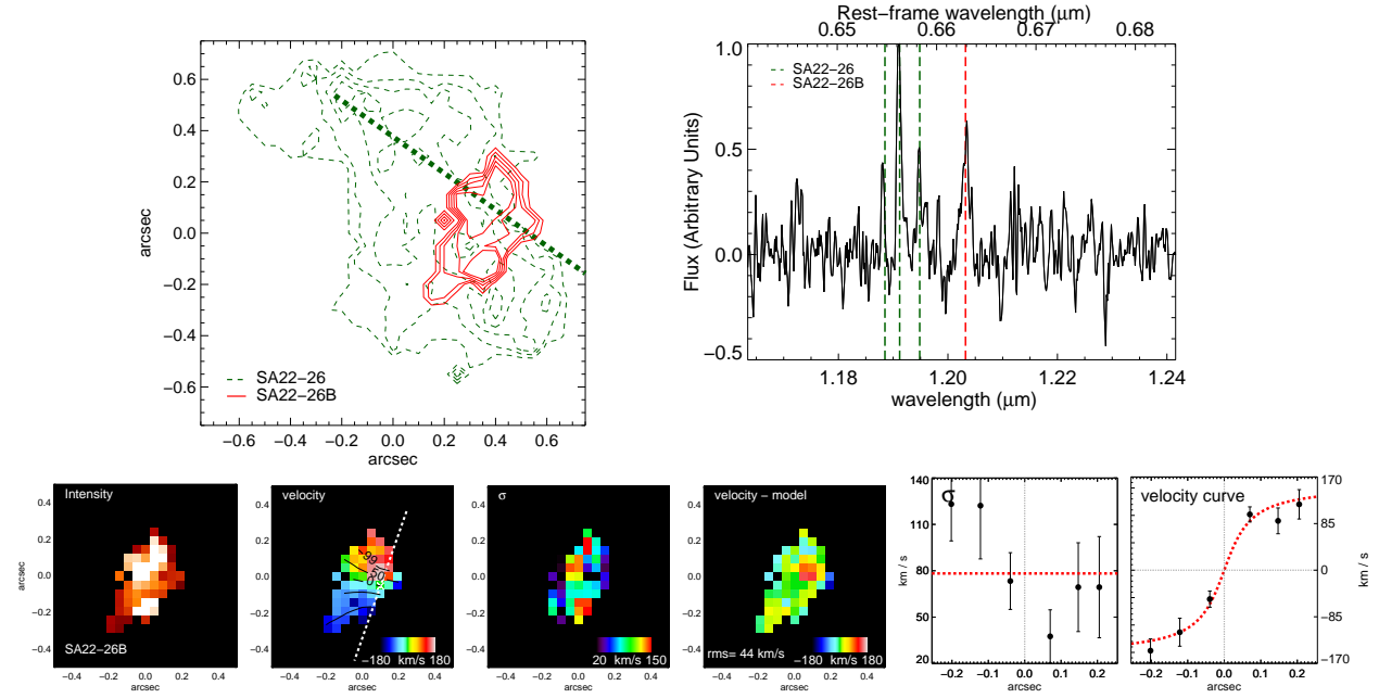
Figure A1. Top Left: Intensity contours of our serendipitous detection (red) and SA22-26 (green-dashed) sources within the SINFONI data-cube. The dashed line shows the position angle derived for SA22-26 source. There is a clear spatially overlap between both emissions. Top Right: Spatially integrated one-dimensional spectra of SA22-26B. The emission is integrated within the red contour showed in top-left figure. The red-dashed line shows the emission line detected at \lambda \sim 1.203 \mu\text{m} . The green-dashed lines show the \text{H}\alpha , [\text{N II}]\lambda\lambda 6583, 6548 emission lines for the SA22-26 source extracted from the same area. Bottom: Intensity, velocity, line-of-sight velocity dispersion ( \sigma ), residual field, one-dimensional velocity dispersion profile and one-dimensional velocity profile (as in Fig. 3) for our serendipitous detection. The spatial scale is showed in arcseconds due to the uncertain redshift determination.
