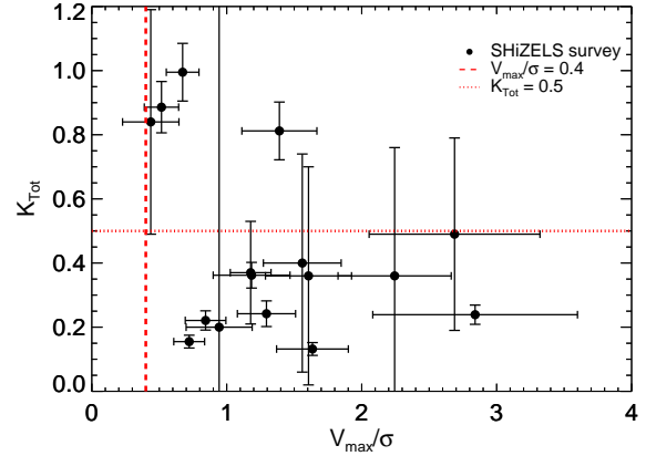
Figure 4. The kinematic measure K_{\text{Tot}} (see §3) against the V_{\max}/\sigma ratio for the SHIZELS Survey. The red-dashed line shows the V_{\max}/\sigma = 0.4 ratio which has been used to crudely differentiate rotating systems from mergers (Förster Schreiber et al. 2009). The red-dotted line shows the K_{\text{Tot}} = 0.5 value which is used to distinguish between galaxy disks from mergers (Shapiro et al. 2008). Although there is no strong correlation between both quantities, it is notable that galaxies classified as mergers by kinemetry criterion tend to show lower V_{\max}/\sigma ratio, however not as low as 0.4. This suggests that the V_{\max}/\sigma = 0.4 criterion tend to underestimate the total number of mergers in a given galaxy sample.
