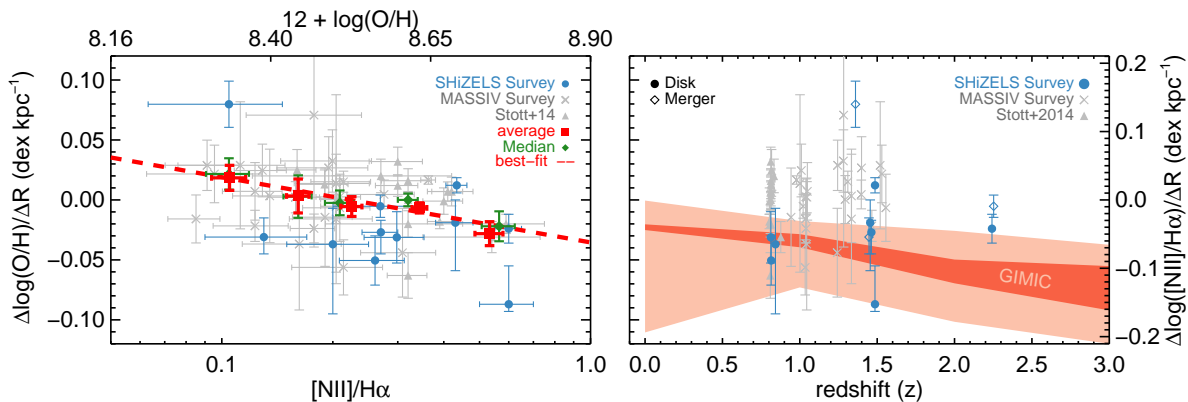
Figure 9. Left: Metallicity gradient as a function of the [N II]/H\alpha emission line ratio from the one-dimensional spectra of each galaxy. The sky blue circles are individual galaxies within the SHiZELS Survey. The grey crosses denotes the sample from the MASSIV Survey (Queyrel et al. 2012) corrected for a Pettini & Pagel (2004) metallicity calibration. The grey triangles denotes the sample from Stott et al. (2014). The red squares and green diamonds show the average and median metallicity content and metallicity gradient per \Delta \log_{10}(O/H)=0.1 bin respectively. The error bars shows 1\sigma uncertainties. Within the literature, we only consider [N II]/H\alpha fluxes ratio above 1\sigma detection threshold. The red-dashed line shows the best linear fit ( \Delta \log_{10}(O/H)/\Delta R = a + b \times \log_{10}(O/H) ) to the average values with a slope value of a = -0.10 \pm 0.04 and zero-point of b = 0.89 \pm 0.30 . The SHiZELS survey supports the anti-correlation such that metallicity gradients tend to be negative in metal-rich galaxies and positive in low-metallicity galaxies (see also Queyrel et al. 2012). Right: Metallicity gradient as a function of redshift. We also show the theoretical evolution of the metallicity gradient with redshift from the GIMIC simulation (Crain et al. 2009; McCarthy et al. 2012). The shaded-red area shows the range of metallicity gradients for all disk galaxies in the simulation in the mass range 9.5 < \log_{10}(M/M_{\odot}) < 11.5 , whilst the shaded light-red denotes the 1\sigma scatter at each epoch. Diamonds and circles show targets classified as Merger and Disk respectively from kinemetry criterion (see §3). The metallicity gradients measured from the SHiZELS survey do not support the evolution predicted from the GIMIC simulation from z = 0 to z = 1.47 .
