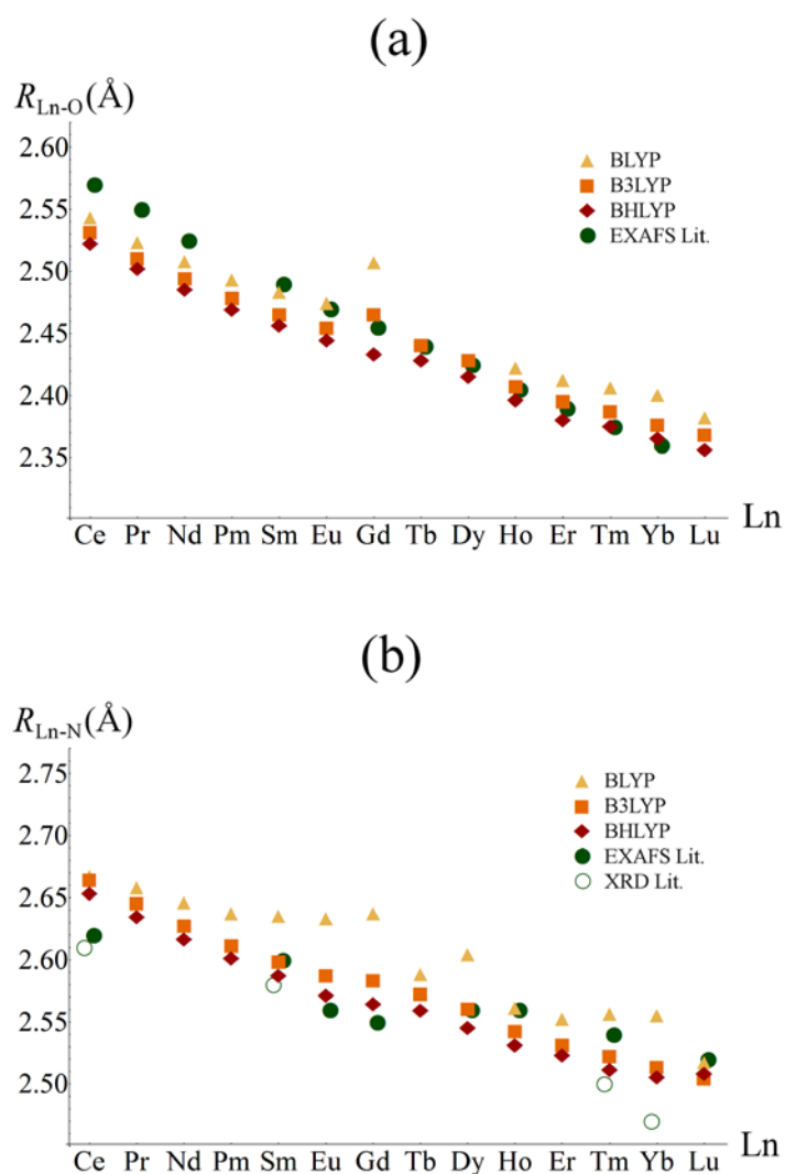
Figure 2. (a): Average Ln-O bond lengths of [\text{Ln}(\text{H}_2\text{O})_9]^{3+} (Ln = Ce – Lu) calculated with DFT (present work) and obtained experimentally via EXAFS 77 ; (b): Average Ln-N bond lengths of [\text{Ln}(\text{BTP})_3]^{3+} calculated with DFT (present work) and obtained experimentally via EXAFS and XRD 15-21 . Literature data has been offset by \pm 0.1 on the x-axis for readability.
