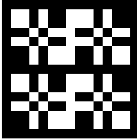
Figure 3: Rank 7 coded-aperture. Transparent and opaque elements are presented in white and black, respectively. With 84 transparent and 85 opaque elements, the modelled aperture yields 49.7% transparency. A frame of 5 mm was added around the 13x13 aperture to represent clear boundaries.
