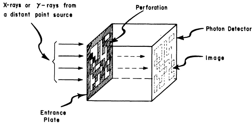
Figure 1: Scatter-hole camera aperture as proposed by Dicke [15].
