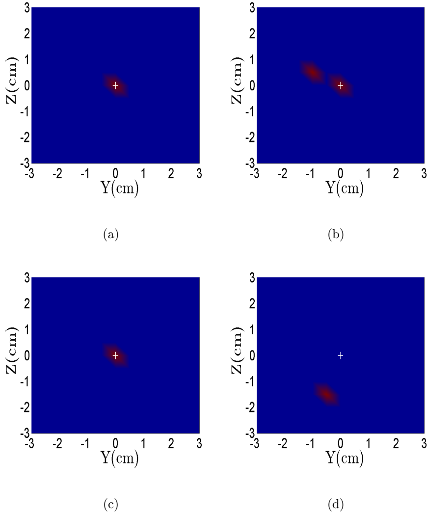
Figure 7: MATLAB plots of MCNPX simulation results with ^{252}\text{Cf} source located 10 cm away from the aperture: (a) ^{113}\text{Cd} aperture, thickness - 10 mm (b) W aperture, thickness - 10 mm, (c) ^{113}\text{Cd} aperture, thickness - 25 mm and (d) W aperture, thickness - 25 mm. White cross marks the actual location of the source.
