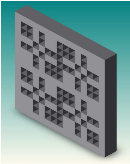
Figure 4: Aperture with the 5 mm frame constructed in MCAM
