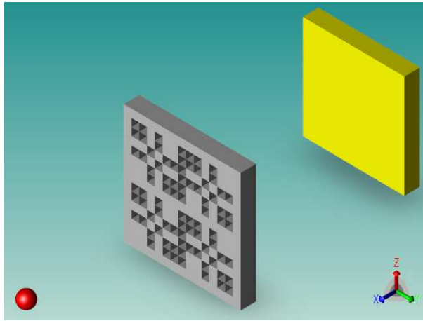
Figure 5: 3D image of the complete MCPNX geometry
