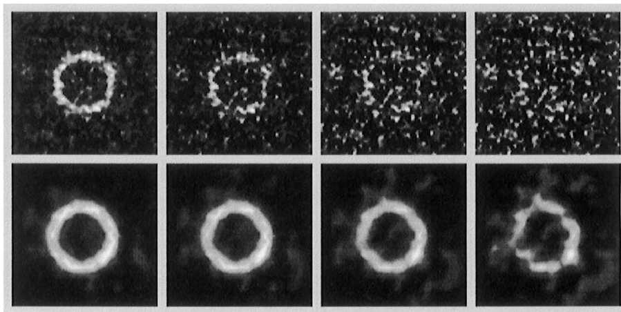
Figure 2: Results of experiments carried out with a circular ^{241}\text{Am} source by Ivanov et al. [50]. Detection time is equal to 8, 4, 2 and 1 of relative units (from left to right).
