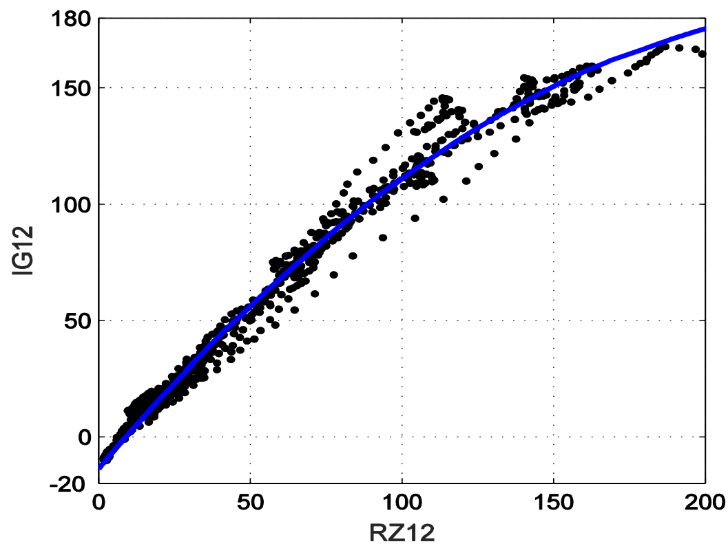
Figure 5. Variation of the monthly average IG values vs the monthly average RZ values. The best fit line is shown as a solid line.
