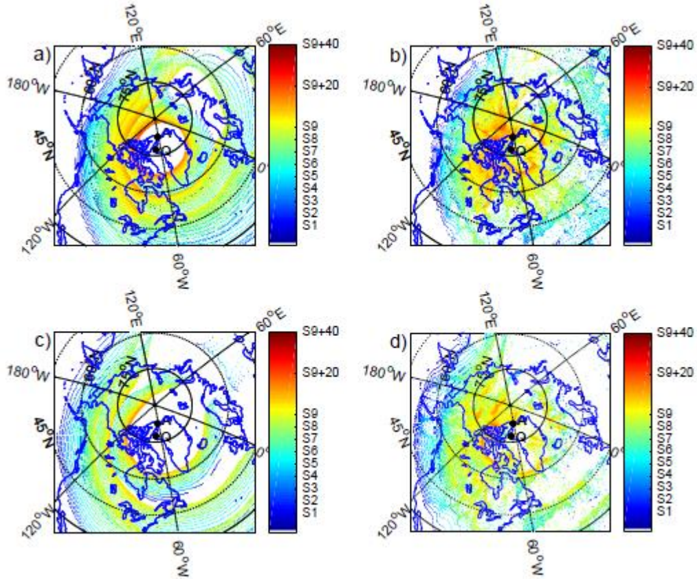
Figure 11. Predicted signal coverage at 8.0 and 11.1 MHz for a transmitter located in Qaanaaq for 23:30 UT on 17 October 2014 using the IRI based model. Frames (a) and (c) are for the background ionosphere, and frames (b) and (d) are for one particular patch scenario. The colours indicate the received signal strength while the position of the transmitter (Qaanaaq) and the receiver (Alert) are marked with Q and A, respectively.
