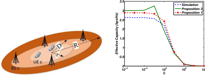
Fig. 1. LHS: A schematic of the system. RHS: The EC of the link versus \theta_c for three BSSs with equal transmission power, N_t = 5 , and \alpha = 4 . The allocated feedback bits are B_{cc} = 8 (distance 300m), B_{cc'} = 6 (distance 400m), and B_{cc''} = 5 (distance 500m).
