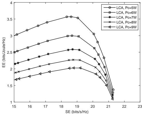
Fig. 10. Energy efficiency vs. spectral efficiency with different circuit power.
