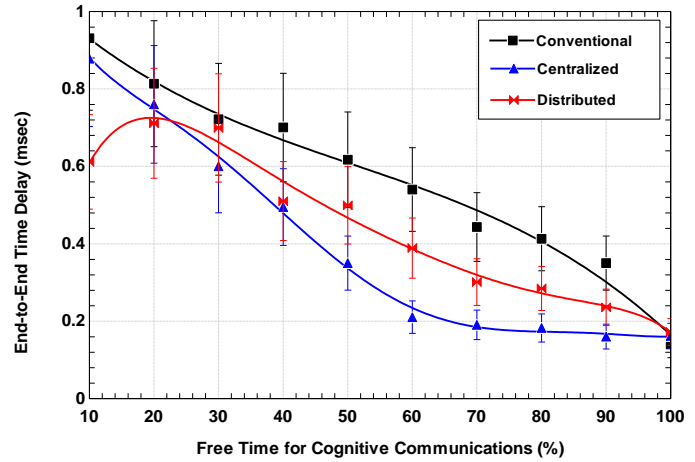
Fig. 10. Cognitive end-to-end time delay vs. free time for cognitive communications.
