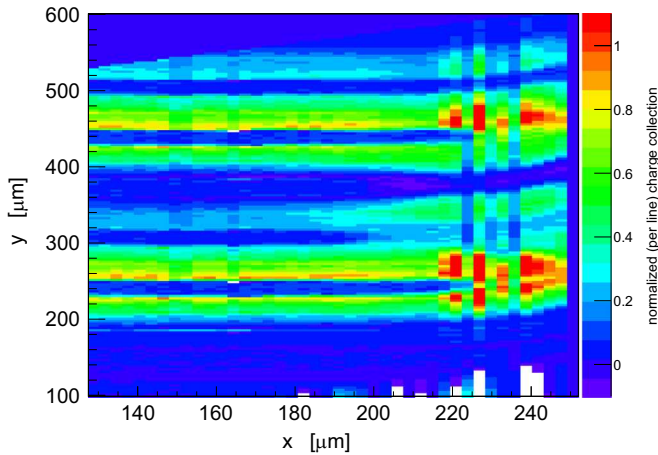
Fig. 9. Performance of a sample irradiated with protons at 2 \times 10^{15} n_{\text{eq}} \text{ cm}^{-2} , DC ganged. Normalized charge collection map of a ganged strip channel.
