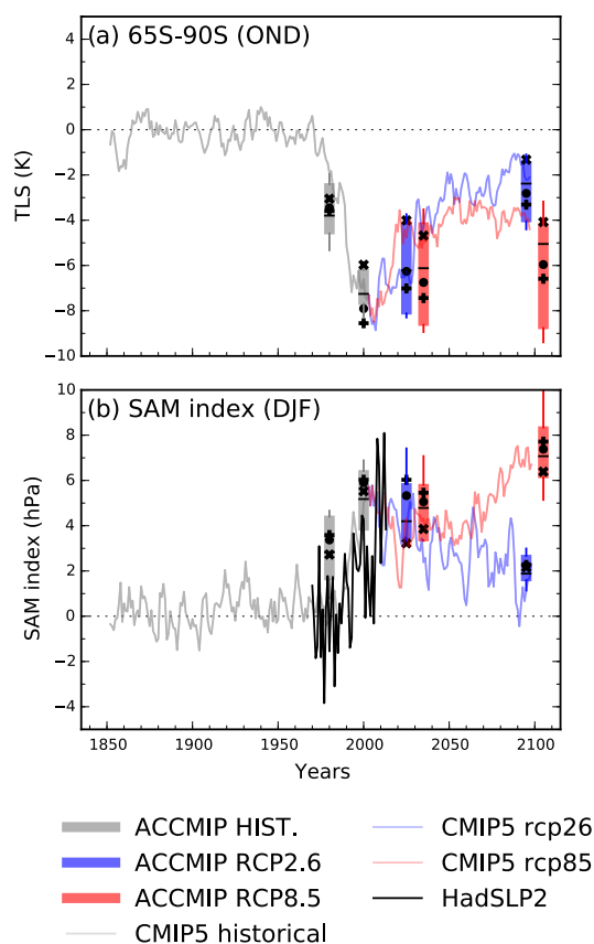
Figure 7. (a) MSU temperature lower stratosphere (TLS) and (b) SAM index time series from 1850 to 2100. The box, whiskers, line, dot, “plus”, and “cross” symbols show the interquartile range, 95 % range, median, multi-model mean, CHEM, and NOCHEM means respectively, for the ACCMIP models. The 5-years average of the CMIP5 multi-model mean is shown. In addition, HadSLP2 observational data set for (b) is represented by a solid black line. The ACCMIP models are normalized to Hist 1850 time slice levels, and the HadSLP2 data set and CMIP5 models are relative to 1860–1899 climatology.
