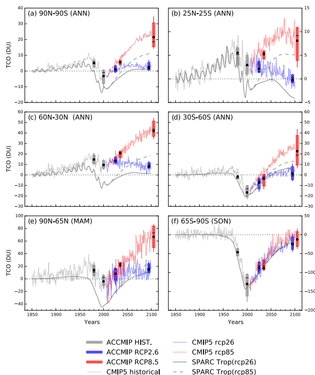
Figure 3. Total column ozone (DU) time series from 1850 to 2100, normalized to Hist 1850 time slice levels. The box, whiskers, and line indicate the interquartile range, 95% range and median respectively, for the ACCMIP CHEM models. In addition, the multi-model mean of the CMIP5 CHEM models and the IGAC/SPARC mean are shown.
