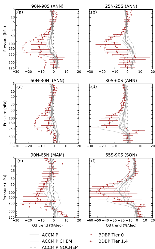
Figure 2. Vertically resolved ozone trends ( \% \text{dec}^{-1} ), for ACCMIP multi-model mean, CHEM and NOCHEM models compared to BDBP Tier 1.4 (regression model fit with uncertainty estimates indicating 95 % confidence intervals, one tail) and Tier 0 (observations).
