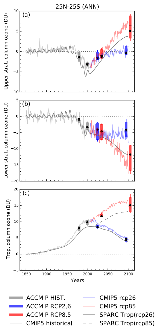
Figure 4. As Fig. 3, but for the upper stratosphere (10–1 hPa), lower stratosphere (> 15 hPa), and tropospheric columns ozone (DU) in the tropics.
