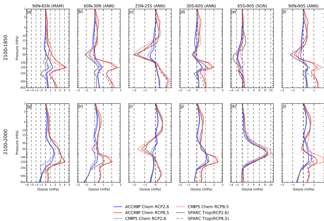
Figure 5. Vertically resolved ozone change between 2100 and 1850 ( a to f ), and 2100 and 2000 ( g to l ) time slices. Figures ( a )–( g ) are for Arctic boreal spring mean, ( b )–( h ) and ( d )–( j ) for NH and SH midlatitudes annual mean respectively, ( c )–( i ) for tropical annual mean, ( e )–( k ) for Antarctic austral spring mean, and ( f )–( l ) for global annual mean.
