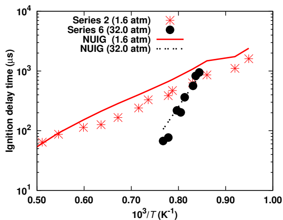
Figure 12: NUIG predictions for bio-syngas combustion [41]
