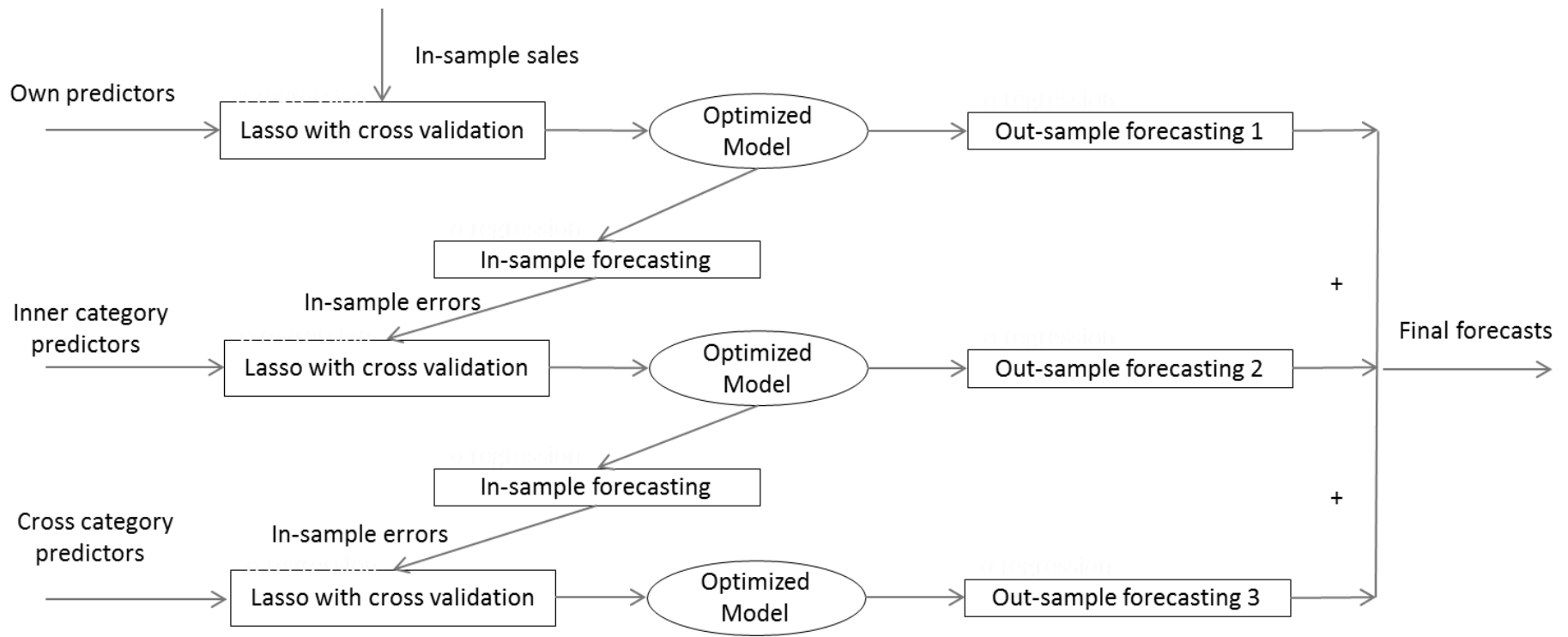
Figure 2 Multistage LASSO process
