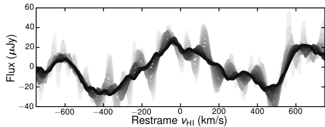
Figure 3. Noise reducing properties of the Savitzky-Golay filter with increasing filter window width demonstrated on the cluster member galaxy stack. Colours of the lines go from lighter to darker shades in increasing window length. The black line at the foreground of the figure is smoother spectrum after applying the final window length choice, \sim 300 \text{ km s}^{-1} , which is also the one we finally applied to the data. Similar results are obtained for the galaxy stacks, as well as their associated noise stacks.
