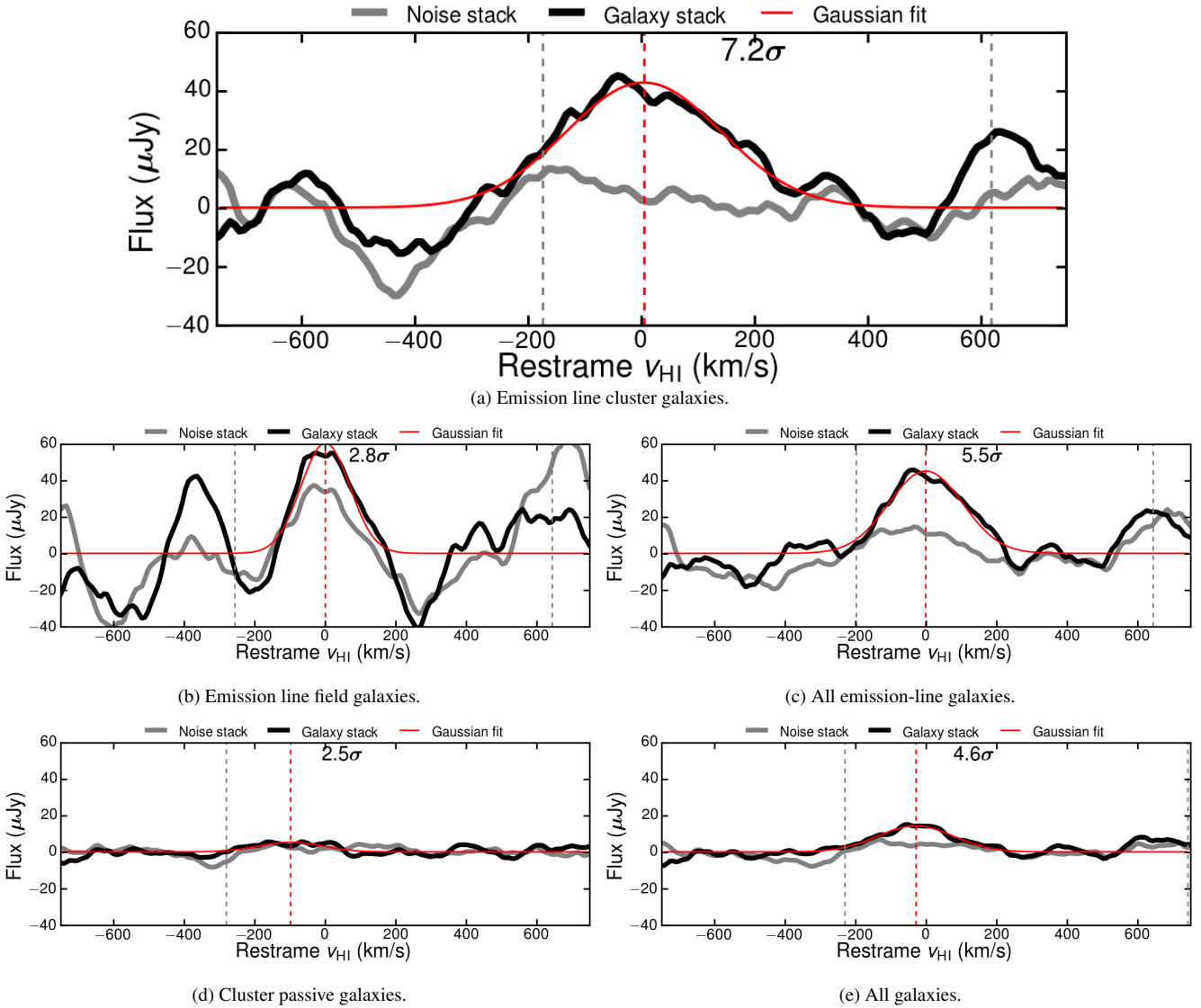
Figure 5. Final HI stacks after filtering and correcting for continuum over-subtraction. The solid black lines show the galaxy stacks and the gray lines show the corresponding noise properties. The thin, solid red lines show the Gaussian fits to the profiles located around a 0 restframe velocity. The vertical, dashed red line show the position of the peak, which is labelled with its significance based on the underlying noise properties. The RMS noise is calculated using only the data between the vertical, dashed gray lines, where at least 80% of the peak number of sources are stacked. Note clear detections of HI are made for the line emitters, while no detections are made in the case of the cluster passive galaxies.
