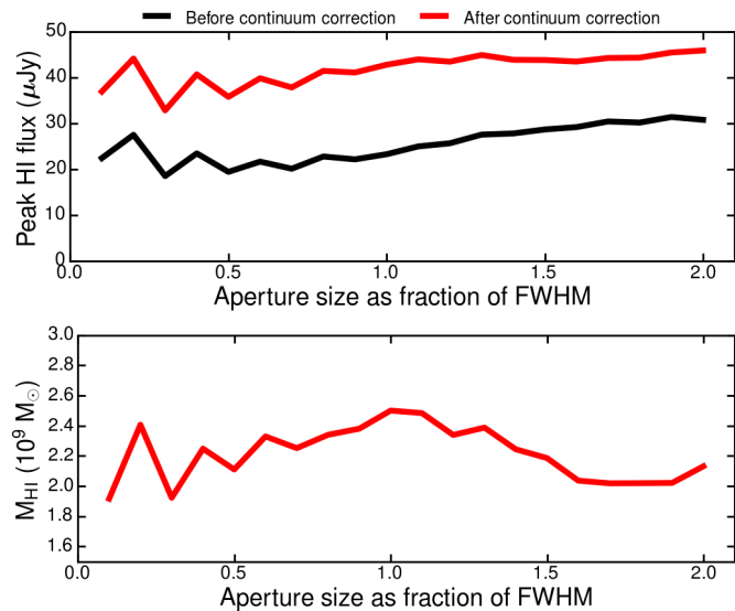
Figure 2. Top: HI peak emission flux in the cluster line emitter stack as function of the aperture size used for extracting the individual spectra. The horizontal scale indicates the fraction by which the aperture width and height are scaled as a function of the FWHM. The trend in the peak emission does not change before and after correcting for the continuum over-subtraction (see §3.3). Bottom: Average HI mass of cluster line emitters (see §3.4), as function of the aperture size used for extracting the individual spectra. The horizontal scale indicates the fraction by which the aperture width and height are scaled as a function of the FWHM.
