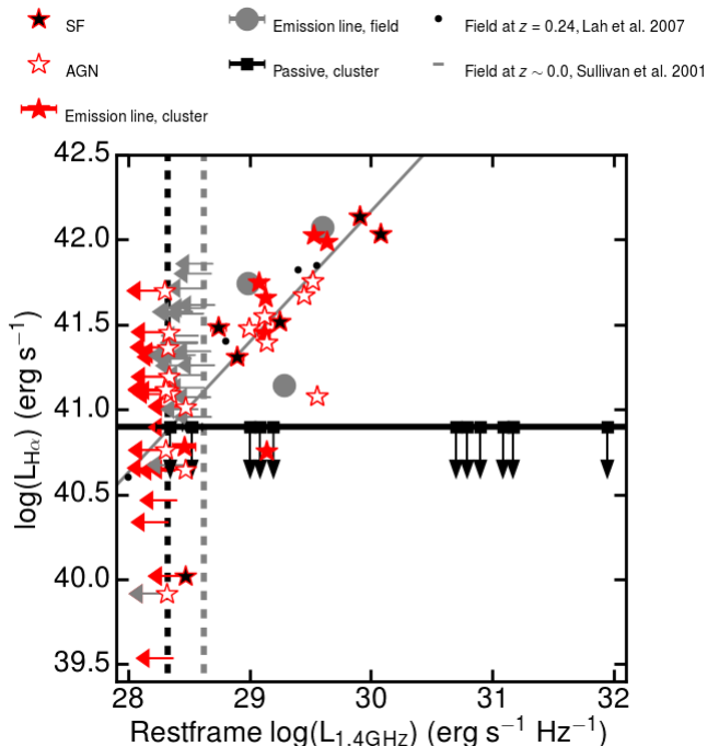
Figure 9. Relationship between H \alpha luminosity and restframe 1.4 GHz radio luminosity. The vertical black dashed line marks the RMS noise at the centre of the radio image, while the gray line represents the detection limit towards the edges of the FOV. The horizontal, solid, black line indicates the detection limit of the H \alpha NB survey. Passive galaxies, undetected in H \alpha , are only plotted if they have a detection in the radio. Error bars are plotted but in most cases they are smaller than the symbol size. On average, the galaxies undergoing SF and optical AGN episodes have lower radio luminosities, probably driven by SNRs, while the passive cluster galaxies host powerful jetted and tailed radio sources. It is noteworthy that, in the case of line emission sources with radio detections the H \alpha luminosity correlates well with the radio luminosity. We overplot for comparison data points for field galaxies at z = 0.24 from Lah et al. (2007) and the linear correlation between H \alpha and radio luminosity for local galaxies found by Sullivan et al. (2001).
