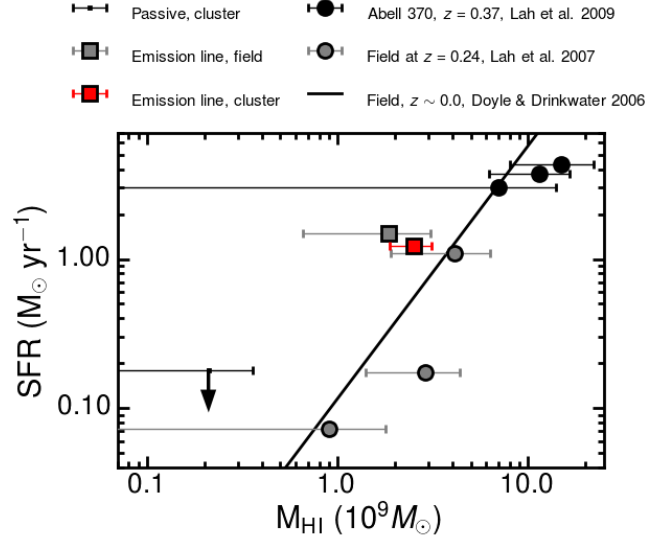
Figure 8. Relationship between SFR and integrated HI mass. All SFRs are calculated with a Chabrier IMF. For the passive population, the SFR is an upper limit. Overplotted are the data points for cluster Abell 370 at z = 0.37 (Lah et al. 2009) and a blank field at z = 0.24 (Lah et al. 2007), together with the SFR- M_{HI} relationship for the local Universe (Doyle & Drinkwater 2006). Note that it is difficult to compare our dataset with other work because of the different ways of measuring the HI mass and the different SF tracers used ( H\alpha , [OII] or IR).
