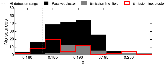
Figure 1. Redshift distribution of sources in each galaxy sample (emission-line cluster members, emission-line field galaxies and cluster passive galaxies). The HI redshift coverage of the WSRT data is marked by the vertical dashed lines.
