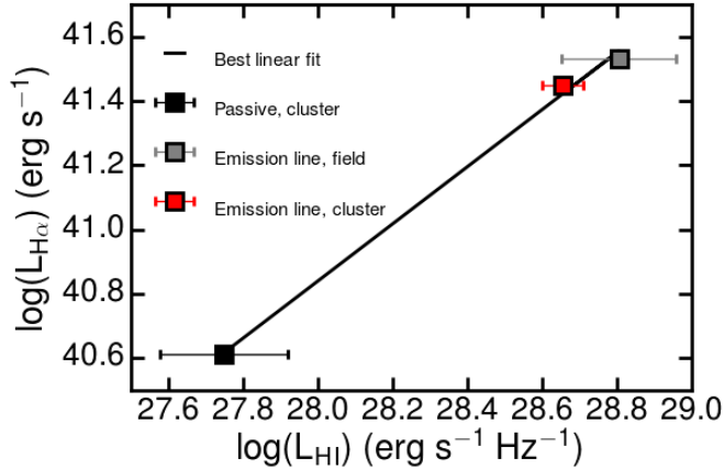
Figure 7. Relationship between H\alpha luminosity and peak HI luminosity. As expected the cluster passive galaxies, selected to be non-line emitters contain less HI than emission-line galaxies. Line emitters are selected to be H\alpha luminous, indicating the presence of vigorous SF and/or AGN activity.
