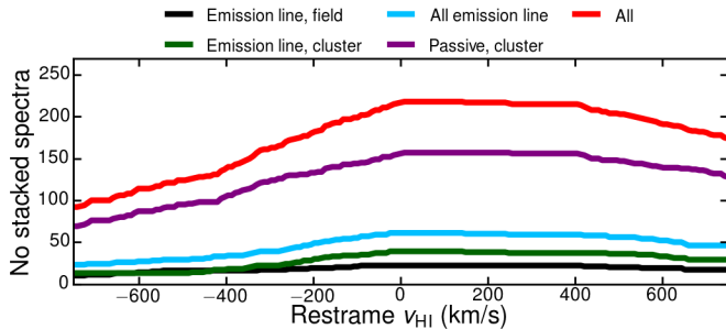
Figure 4. Number of sources stacked in each velocity channel, for the separate stacks. The passive cluster galaxy stack (purple line) benefits from a factor of > 5 more sources than the stacks for the H\alpha line emitters (mostly star-forming and some AGN) galaxies inside (green line) and outside the cluster (black line). Note how the number of sources dwindles towards the edges of the WSRT HI bandpass. The asymmetry in the number of sources is caused by the redshift distribution of the stacked sources (see Figure 1), preferentially located at redshifts lower than the central WSRT HI coverage.
