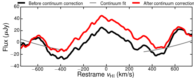
Figure 6. Correction for the continuum over-subtraction in the case of the cluster line emitter HI stack.
