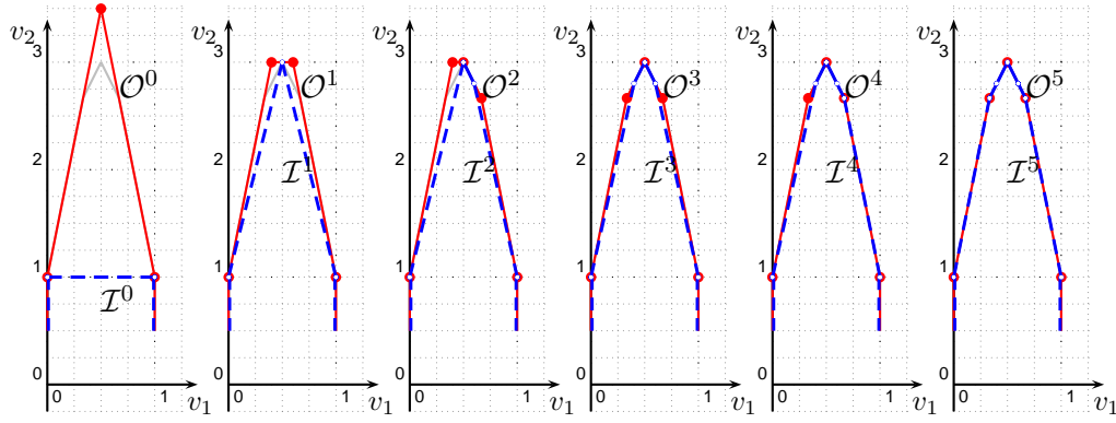
Figure 3. The shrinking of \mathcal{O}^k and the enlargement of \mathcal{I}^k with iteration k .
