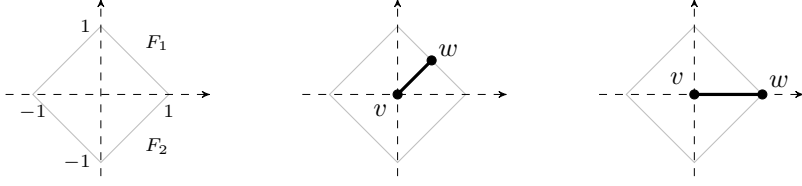
FIGURE 1. An infinitesimally flexible and an infinitesimally rigid placement of K_2 in (\mathbb{R}^2, \|\cdot\|_1) .
