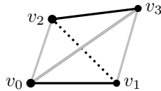
FIGURE 2. A framework colouring for an infinitesimally rigid placement of K_4 in (\mathbb{R}^2, \|\cdot\|_{\mathcal{P}})
