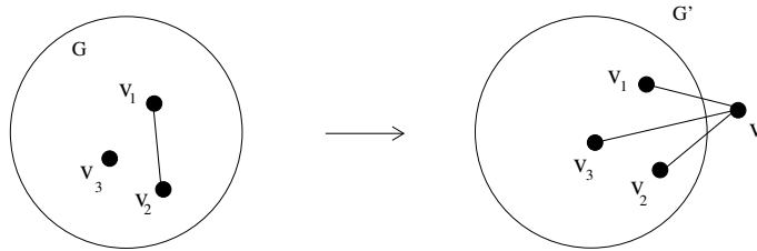
FIGURE 1. The Henneberg 2 move.
