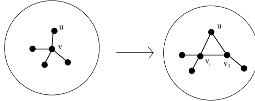
FIGURE 3. The vertex splitting move.
