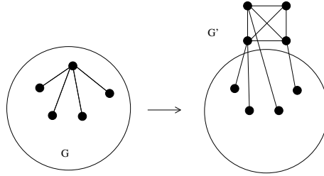
FIGURE 2. The vertex-to- K_4 move.
