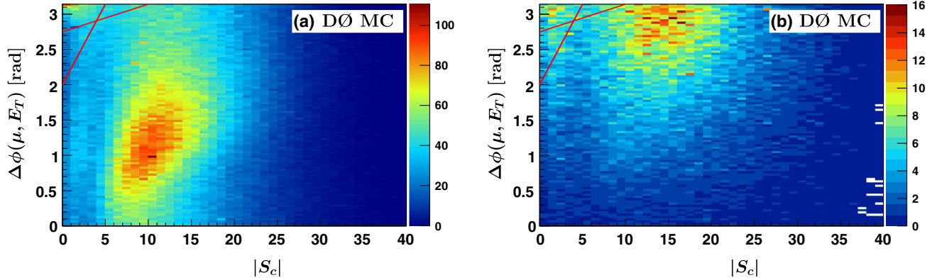
FIG. 1 (color online). The |S_c| versus \Delta\phi(\mu, E_T) plane for (a) t\bar{t} events and (b) for W + \text{jets} background events. The selection requirements are indicated by the solid lines.
