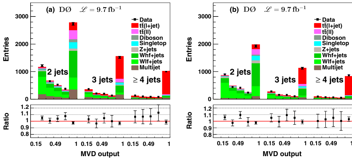
FIG. 2 (color online). Distributions of the MVD b identification output distribution for the \ell + 2 jets, \ell + 3 jets and \ell + \geq 4 jets data sample in the (a) e + \text{jets} and (b) \mu + \text{jets} decay channel. The data are compared to the sum of predicted contributions from signal and background processes. More details on how the sample composition is derived can be found in the text.
