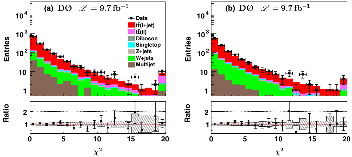
FIG. 5 (color online). Distribution of \chi^2 for the best solution with lowest \chi^2 for the (a) e + \text{jets} and (b) \mu + \text{jets} final states. The data are compared to the sum of predicted contributions from signal and background processes. The signal contribution is derived employing MC@NLO simulated events normalized to the measured inclusive t\bar{t} cross section of 8.0 pb. The highest bin in the histograms is used as an overflow bin. The ratios of data to the sum of the signal and all background contributions are shown in the panels below the distributions. The bands show the 1 s.d. combined systematic uncertainties on the sum of the signal and background contributions.
