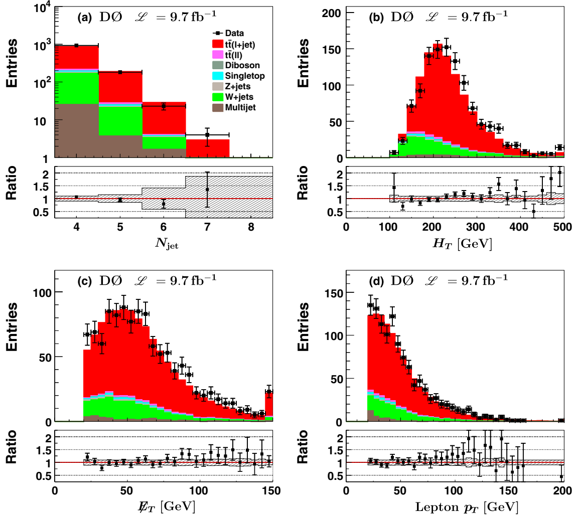
FIG. 4 (color online). Distributions of (a) the number of jets, (b) the scalar sum of the p_T values of the lepton and jets, (c) E_T , and (d) lepton p_T for the \mu + \text{jets} final state. The data are compared to the sum of predicted contributions from signal and background processes. The signal contribution is derived employing MC@NLO simulated events normalized to the measured inclusive t\bar{t} cross section of 8.0 pb. The highest bin in the histograms is used as an overflow bin. The ratios of data to the sum of the signal and all background contributions are shown in the panels below the distributions. The bands show the 1 s.d. combined systematic uncertainties on the sum of the signal and background contributions.
