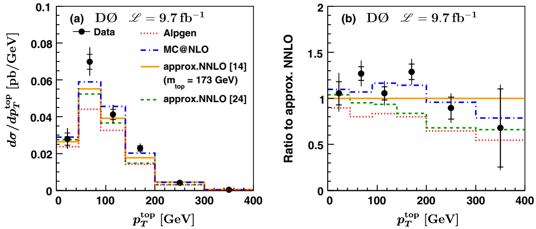
FIG. 11 (color online). (a) Measured differential cross section as a function of p_T^{\text{top}} for data compared to several QCD predictions. The inner error bars correspond to the statistical uncertainties and the outer error bars to the total uncertainties. (b) Ratio of data, ALPGEN (dashed line) and MC@NLO cross sections (dash-dotted line) to the QCD prediction at approximate NNLO [14]. MC simulations and pQCD predictions use a top quark mass of 172.5 GeV unless indicated to the contrary. Note that the correlated overall normalization uncertainty on the differential data points is about \pm 6.6\% .
