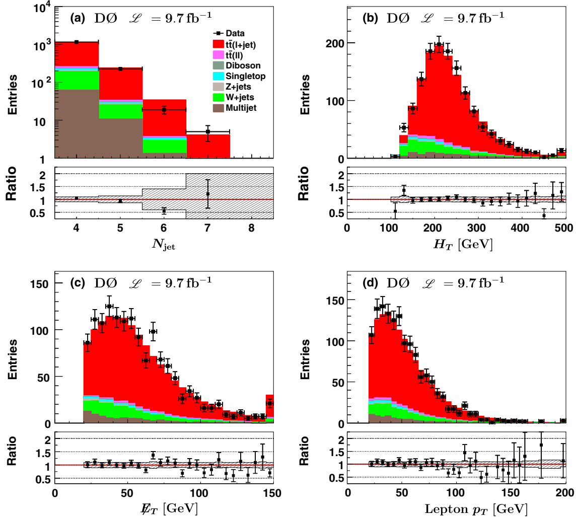
FIG. 3 (color online). Distributions of (a) the number of jets, (b) the scalar sum of the p_T values of the lepton and jets, (c) E_T , and (d) lepton p_T for the e + \text{jets} final state. The data are compared to the sum of predicted contributions from signal and background processes. The signal contribution is derived employing MC@NLO simulated events normalized to the measured inclusive t\bar{t} cross section of 8.0 pb. The highest bin in the histograms is used as an overflow bin. The ratios of data to the sum of the signal and all background contributions are shown in the panels below the distributions. The bands show the 1 s.d. combined systematic uncertainties on the sum of the signal and background contributions.
