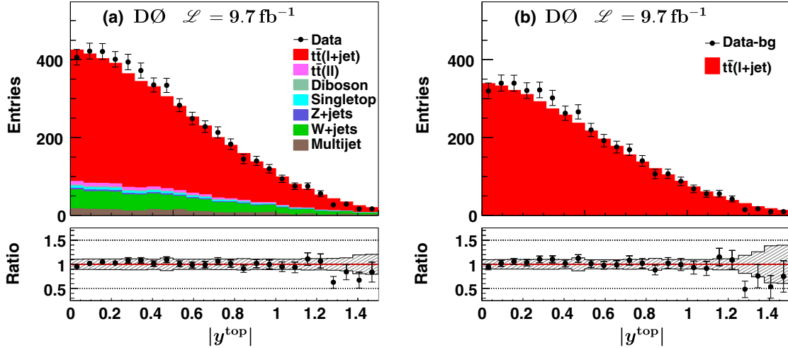
FIG. 7 (color online). Distribution of |y^{\text{top}}| , (a) compared to the sum of predicted contributions from signal and background processes, and (b) the background-subtracted distribution. The signal contribution is derived employing MC@NLO simulated events normalized to the measured inclusive t\bar{t} cross section of 8.0 pb. The lower panels indicate the ratio of the data to (a) the sum of the signal and all background processes, and (b) to the signal process only.
