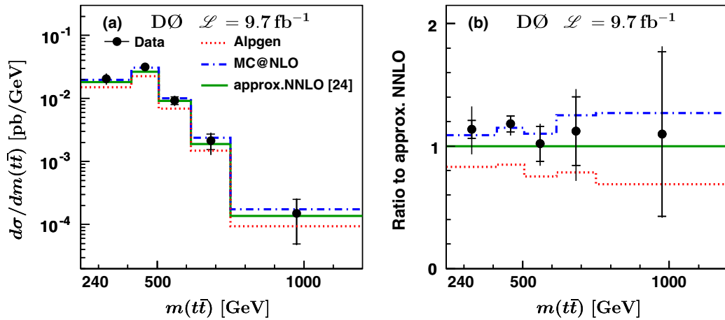
FIG. 9 (color online). (a) Measured differential cross section as a function of m(t\bar{t}) for data compared to several QCD predictions. The inner error bars correspond to the statistical uncertainties and the outer error bars to the total uncertainties. (b) Ratio of data, ALPGEN (dashed line) and MC@NLO cross sections (dash-dotted line) to the QCD prediction at approximate NNLO [24]. MC simulations and pQCD predictions use a top quark mass of 172.5 GeV unless indicated to the contrary. Note that the correlated overall normalization uncertainty on the differential data points is about \pm 6.6\% .
