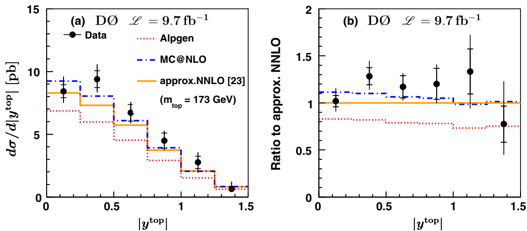
FIG. 10 (color online). (a) Measured differential cross section as a function of |y^{\text{top}}| for data compared to several QCD predictions. The inner error bars correspond to the statistical uncertainties and the outer error bars to the total uncertainties. (b) Ratio of data, ALPGEN (dashed line) and MC@NLO cross sections (dash-dotted line) to the QCD prediction at approximate NNLO [23]. MC simulations and pQCD predictions use a top quark mass of 172.5 GeV unless indicated to the contrary. Note that the correlated overall normalization uncertainty on the differential data points is about \pm 6.6\% .
