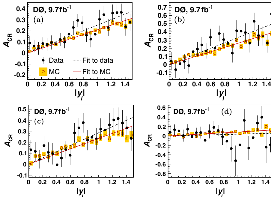
FIG. 6 (color online). The asymmetry of leptons from W + jets production as a function of |y_l| for (a) the inclusive sample, (b) 20 \leq p_T^l < 35 GeV, (c) 35 \leq p_T^l < 60 GeV, and (d) p_T^l \geq 60 GeV. The points show the data from the control region, after the subtraction of the non- W + jets contributions, and the dashed line shows a fit to the functional form y = ax . The empty circles and solid line show the nominal W + jets simulation and its fit to the same functional form. The error bars and shaded regions indicate the statistical uncertainties on the data and simulation.
