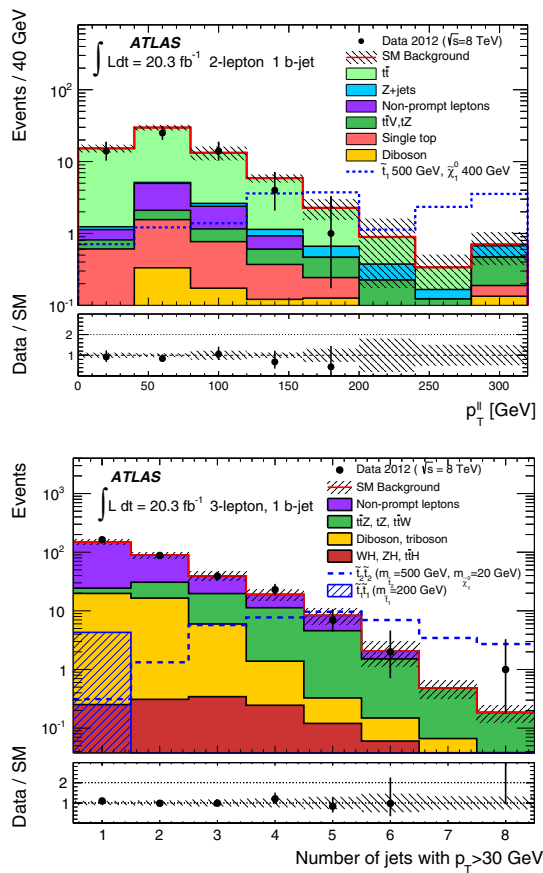
Fig. 1 Top, p_T(\ell\ell) distributions in SR2A before the p_T(\ell\ell) > 80 GeV and \Delta\phi^{\ell\ell} < 1.5 selections. Bottom, number of signal jets with p_T > 30 GeV in events with 3 signal leptons after the lepton, m_{\ell\ell} and b -jets selections in SR3A. Shaded bands denote the background statistical and systematic uncertainty. For illustration, distributions for selected signal points are also shown: the stop natural GMSB model with m_{\tilde{t}_1} = 500 GeV, m_{\tilde{\chi}_1^0} = 400 GeV (top) and the simplified model with m_{\tilde{t}_2} = 500 GeV, m_{\tilde{t}_1} = 200 GeV and m_{\tilde{\chi}_1^0} = 20 GeV for both direct \tilde{t}_2 and \tilde{t}_1 pair production (bottom). The last bin includes the histogram overflow
