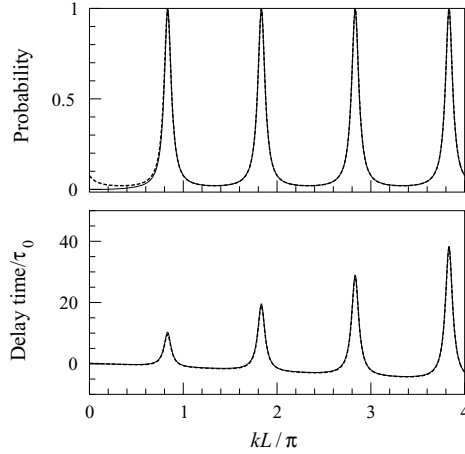
Fig. 3 – Transmission probability T (upper panel) and delay time \tau in units of \tau_0 = \hbar/\varepsilon (lower panel), as a function of kL/\pi . The solid curve is the result for the quantum obstacle with scattering strength U = \infty and \Delta/\varepsilon = 4 , the dashed curve (nearly indistinguishable from the solid curve) the result for the conventional Fabry-Perot interferometer (two fixed classical barriers) from eq. (5) with U/k = 2\sqrt{3} .
