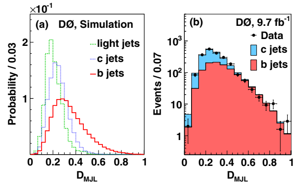
FIG. 1 (color online). (a) The probability densities of the D_{\text{MJL}} discriminant, normalized to unity, for b , c , and light jets passing the final selection requirements. These templates are obtained from MC simulations. (b) The D_{\text{MJL}} discriminant distribution of events in the combined sample after background subtraction. The distributions of the b and c jets are weighted by the fractions found from the fit. Uncertainties are statistical only.
