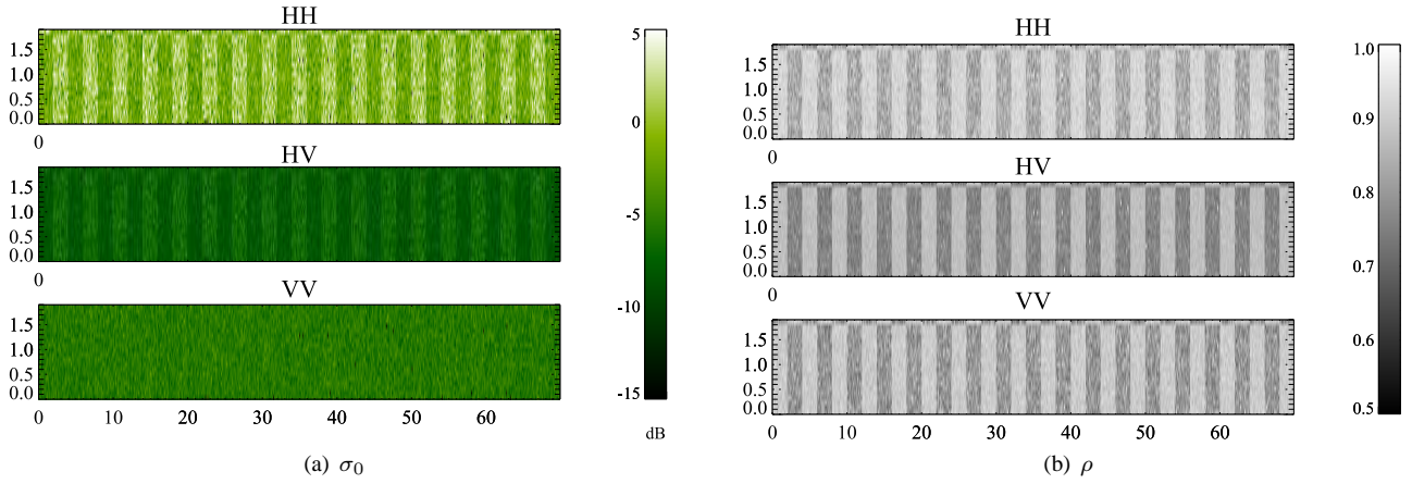
Figure 2. Left: example of SGM generated reflectivity maps showing the HH, HV, and VV channels, respectively, of the first PolInSAR acquisition. Right: corresponding interferometric coherences for the HH, HV, and VV channels, respectively.
