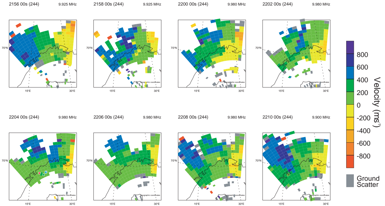
Fig. 10. Two-dimensional maps of the CUTLASS Finland flow data over the interval 21:56–22:10 UT. Cluster footpoint location is indicated in the 22:04 plot.
