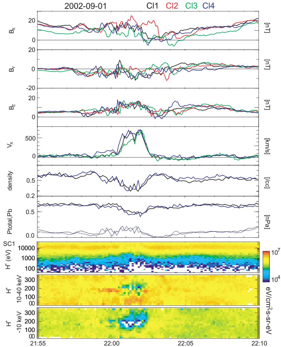
Fig. 3. X , Y and Z component of the magnetic field from the four Cluster spacecraft, X component of the ion flows from Clusters 1, 3, and 4, and proton density and pressures obtained by Clusters 1 and 4 between 21:55 and 22:10 UT. The thick lines in the pressure panel represent to the total pressure, whereas the thin lines the magnetic field pressure. The bottom three panels show the proton energy spectra, pitch angle distribution of high energy (10–40 keV) and low energy (100 eV–10 keV) protons for Cluster 1.
