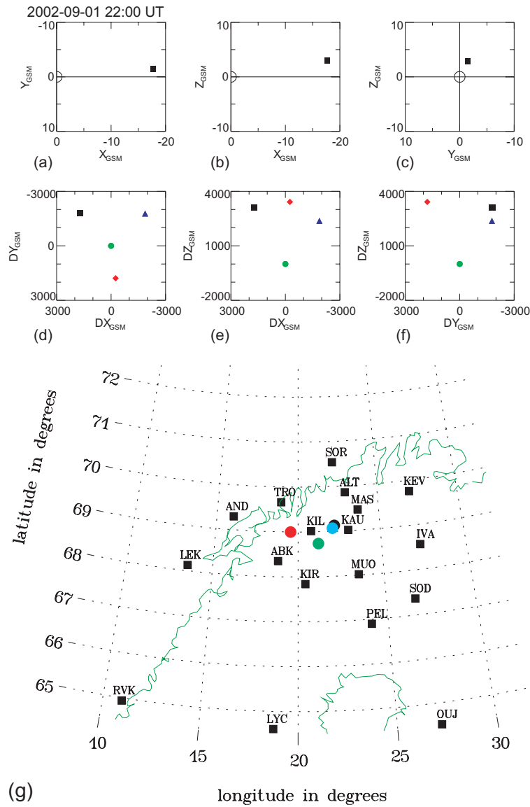
Fig. 1. Location of the four Cluster spacecraft in (a) X – Y plane and (b) X – Z , plane and (c) Y – Z plane, and location relative to the reference spacecraft (CI 3) in (d) X – Y plane and (e) X – Z , plane and (f) Y – Z plane in the GSM coordinates. (g) Location of the MIRACLE stations and that of the Cluster footprints in geographic coordinates. Clusters 1, 2, 3 and 4 data are indicated with black, red, green, and blue, respectively.
