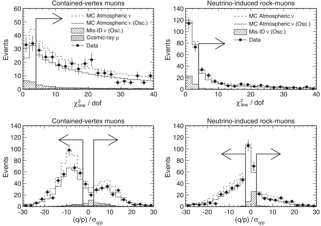
FIG. 9. Distributions of track fit uncertainty, (q/p)/\sigma_{q/p} , and track straightness variable, \chi_{line}^2/dof , used to select events with well-measured muon charge sign. The distributions are plotted for contained-vertex muons (left panels), and neutrino-induced rock-muons (right panels). In each plot, the dashed line indicates the total prediction in the absence of oscillations; the solid line shows the prediction for oscillations with \Delta m^2 = 2.32 \times 10^{-3} \text{ eV}^2 and \sin^2 2\theta = 1.0 ; the shaded histogram shows the cosmic-ray muon background; and the points show the observed data. In addition, the hatched histograms show the component with misidentified charge sign. The arrows indicate the selections used to identify events with well-measured charge sign.
