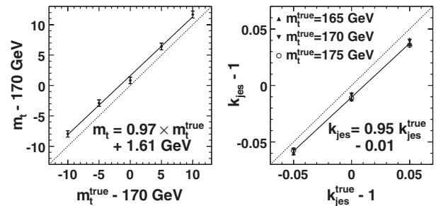
FIG. 2. Mean values of m_t and k_{\text{jets}} from ensemble tests versus true values parameterized by straight lines. Dashed lines represent identical fitted and true values.
