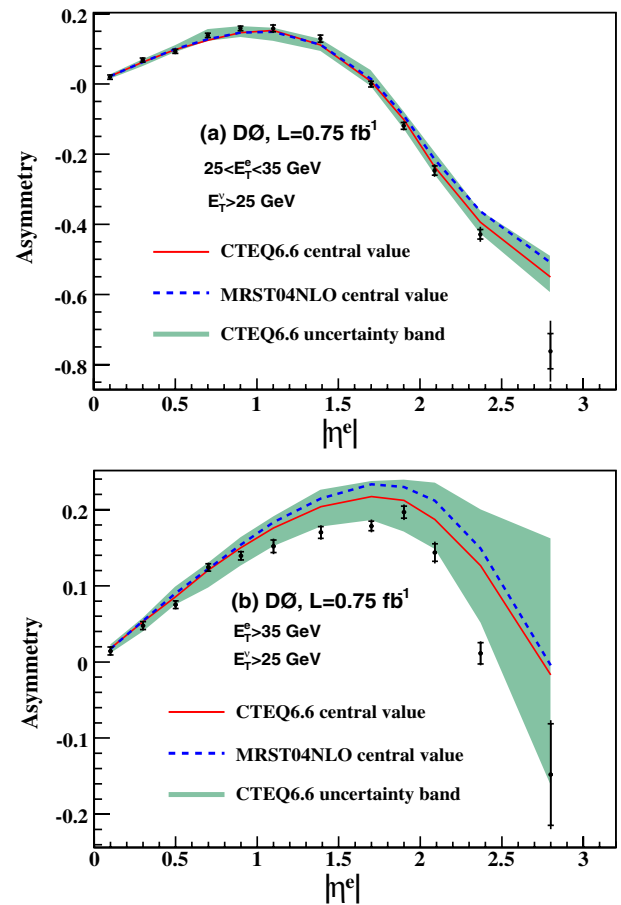
FIG. 2 (color online). The folded electron charge asymmetry distribution in two electron E_T bins: 25 < E_T < 35 GeV for (a) and E_T > 35 GeV for (b). In each plot, the horizontal bars show the statistical uncertainty and the full vertical lines show the total uncertainty on each point. The total uncertainty is the sum in quadrature of the statistical and systematic uncertainties. The solid (dashed) line is the theoretical prediction for the asymmetry using the CTEQ6.6 (MRST04NLO) central PDF set. The shaded band is the uncertainty band determined using the 44 CTEQ6.6 PDF uncertainty sets. All three were determined using RESBOS with PHOTOS.
