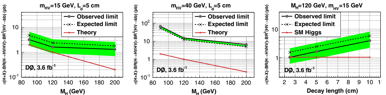
FIG. 4 (color online). The expected and observed 95% C.L. limits on \sigma(H + X) \times \text{BR}(H \rightarrow \text{HV HV}) \times \text{BR}^2(\text{HV} \rightarrow b\bar{b}) for each M_H studied, m_{HV} = 15, 40 GeV, and various values of \nu -hadron L_d . The band shows \pm 1 standard deviation on the expected limit. The reference Higgs boson cross section from the SM [11] is shown, which assumes 100% for \text{BR}(H \rightarrow \text{HV HV}) and \text{BR}(\text{HV} \rightarrow b\bar{b}) .
