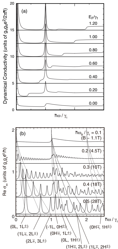
FIG. 12. Interband part of the dynamical conductivity of bilayer graphene plotted against the frequency \omega , in (a) zero magnetic field with different \epsilon_F 's [229] (b) several magnetic fields with \epsilon_F = 0 [230]. Dashed curves in (b) indicate the transition energies between several Landau levels.
