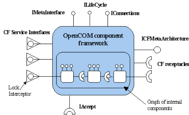
Fig. 2. The Component Framework Model
