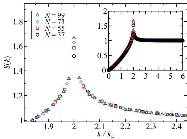
FIG. 6. (Color online) The SSF of the infinitely thin wire at several system sizes. The data shown are extrapolated estimates [2S_{\text{DMC}}(k) - S_{\text{VMC}}(k)] for r_s = 2 a.u.. The main plot shows the behavior at the peak and the inset shows a zoomed-out view. The PCF was not extended beyond L/2 .
