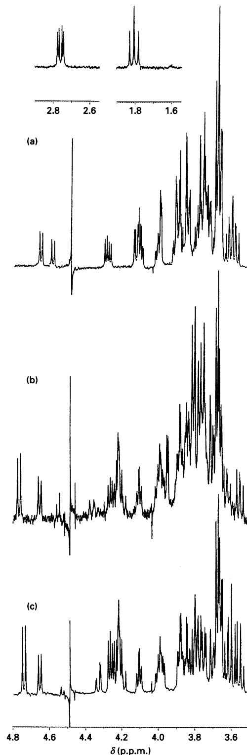
Figure 7 Partial 500 MHz n.m.r. spectra of reduced KS chain fragments isolated from bovine tracheal cartilage and subjected to keratanase digestion
