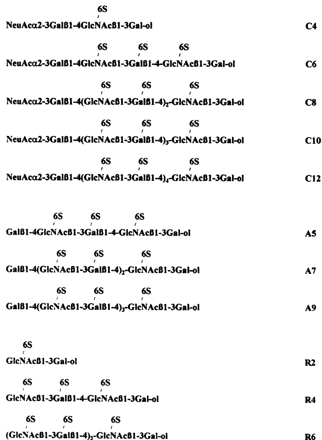
Figure 6 Oligosaccharides derived from the N-linked KS chains attached to fibromodulin from bovine tracheal cartilage which have been isolated and characterized in this study
