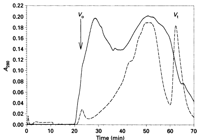
Figure 1 Superose 6 size-exclusion chromatography
