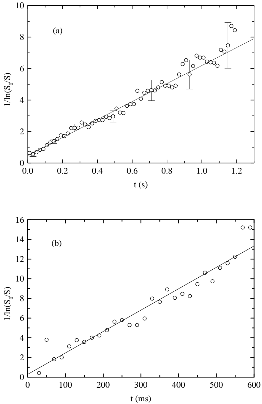
Fig. 9. Plots of (\ln S_0 - \ln S)^{-1} versus time t for hydrodynamically created vortices...
