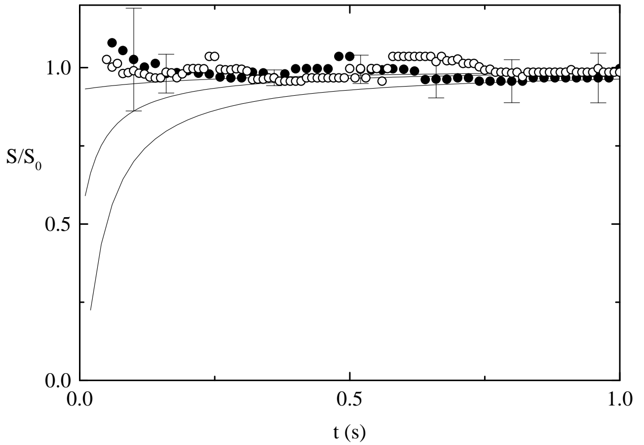
Fig. 11. Comparison of the measured evolution of the second sound amplitude (data points) with those calculated (curves) on the assumption of different initial vortex line densities L_i immediately after the expansion.
