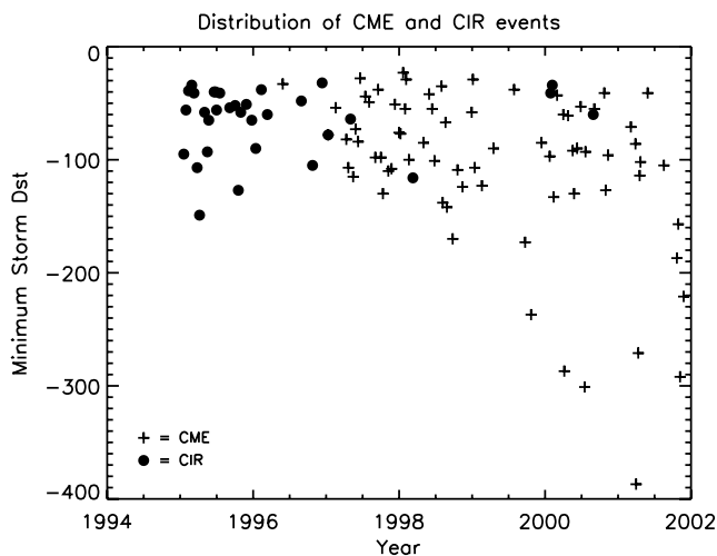
Figure 1. The distribution of ICME events and CIR events used in this study. Most CIR events occur in the declining phase of the solar cycle while ICMEs are most probable close to solar maximum. ICME events typically produce a greater signature in Dst.
