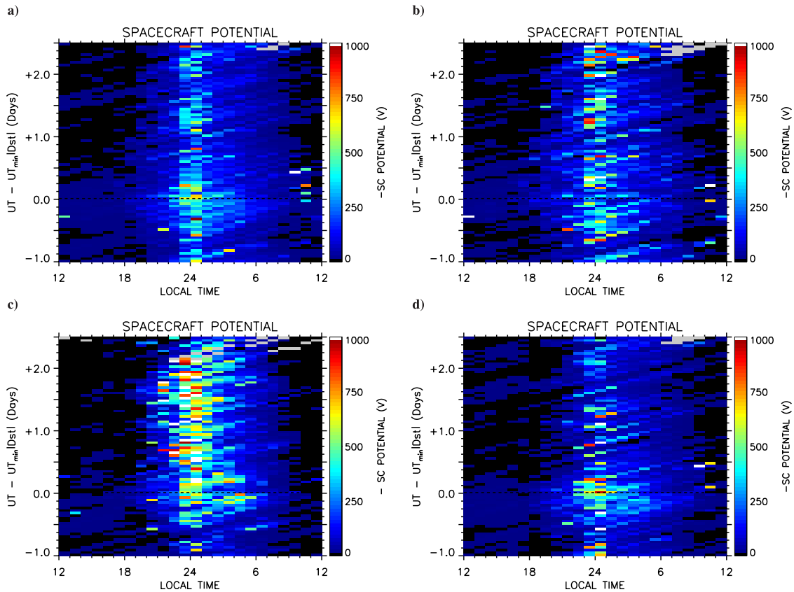
Figure 5. The averaged (negative) spacecraft potential for (a) Group A - all 78 ICME events, (b) Group B - 45 ICME events with minimum Dst > -100 , (c) Group C - 32 CIR events, and (d) Group D - 33 ICME storms with minimum Dst < -100 , as a function of epoch time and local time. The magnitude of the spacecraft potential is much greater for the CIR events, compared with ICME events.
