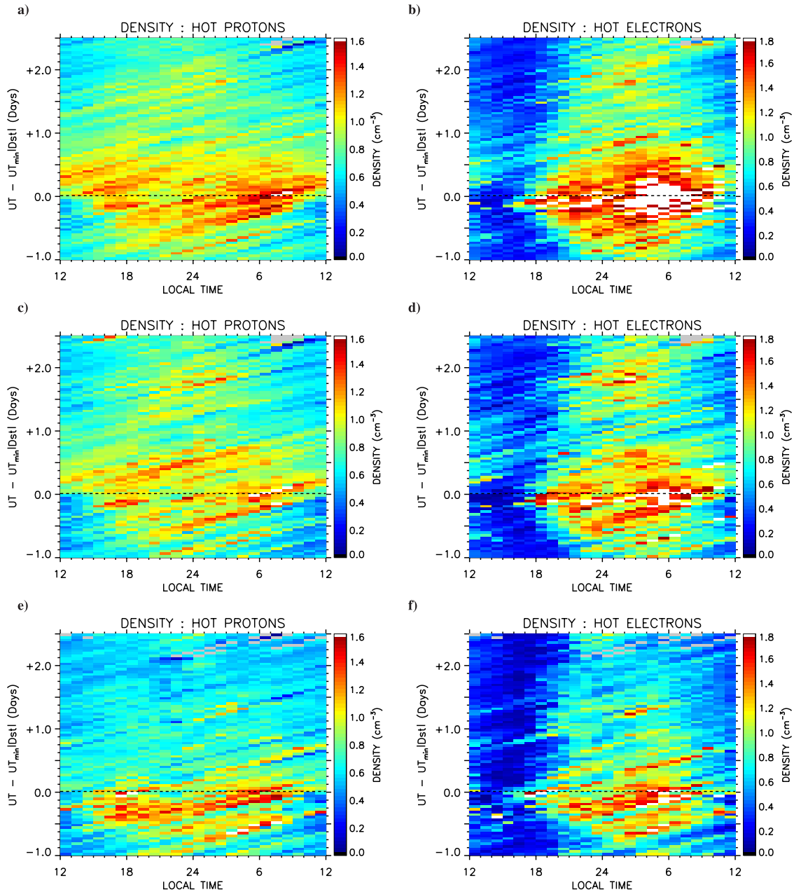
Figure 3. The hot ion and hot electron densities for the three data sets used in the study; (a) and (b) Group A - all 78 ICME events, (c) and (d) Group B - 45 ICME events with minimum Dst > -100 , and (e) and (f) Group C - 32 CIR events, as a function of epoch time and local time.
