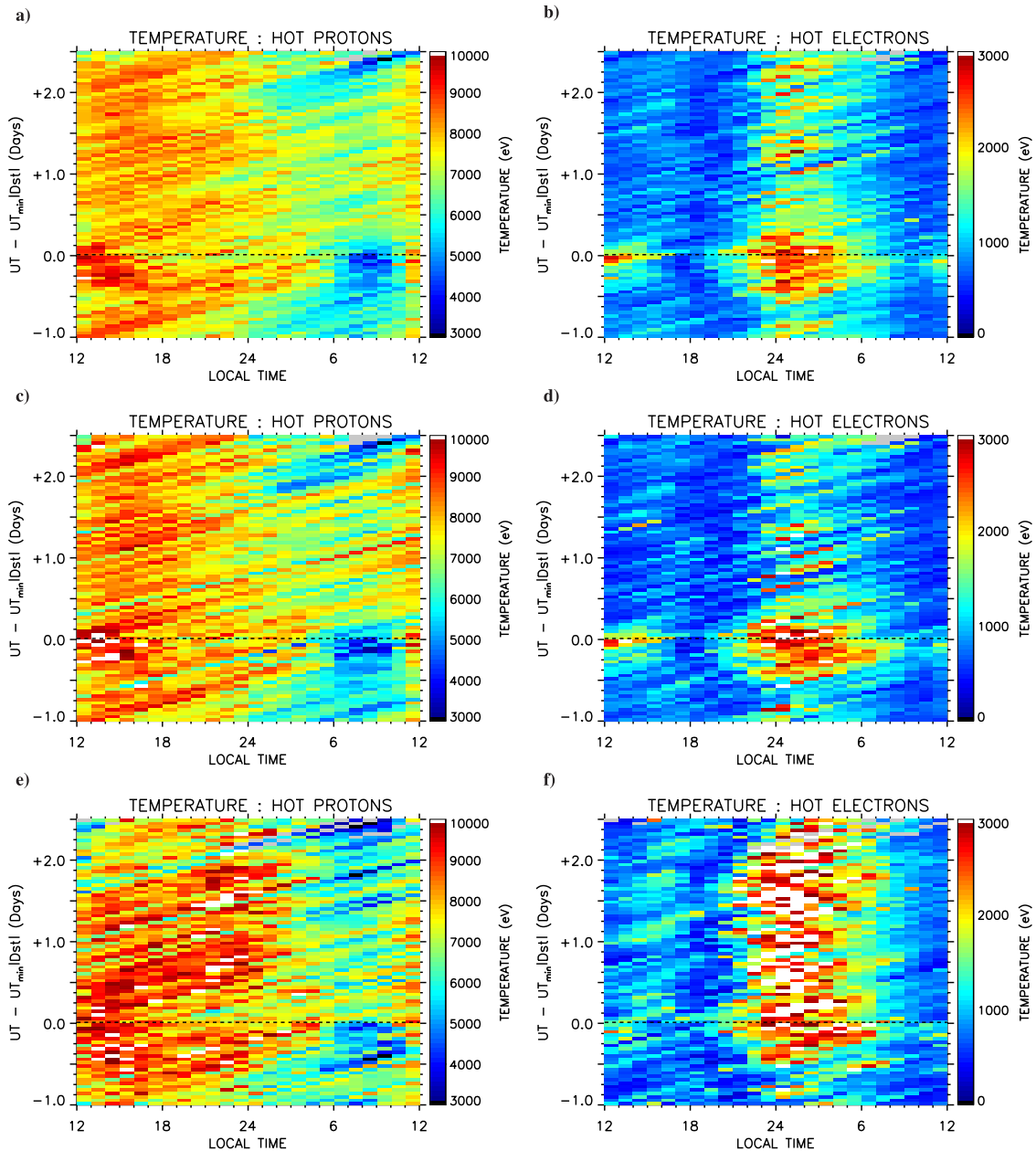
Figure 4. The hot ion and hot electron temperatures for the three data sets used in the study; (a) and (b) Group A - all 78 ICME events, (c) and (d) Group B - 45 ICME events with minimum Dst > -100, and (e) and (f) Group C - 32 CIR events, as a function of epoch time and local time.
