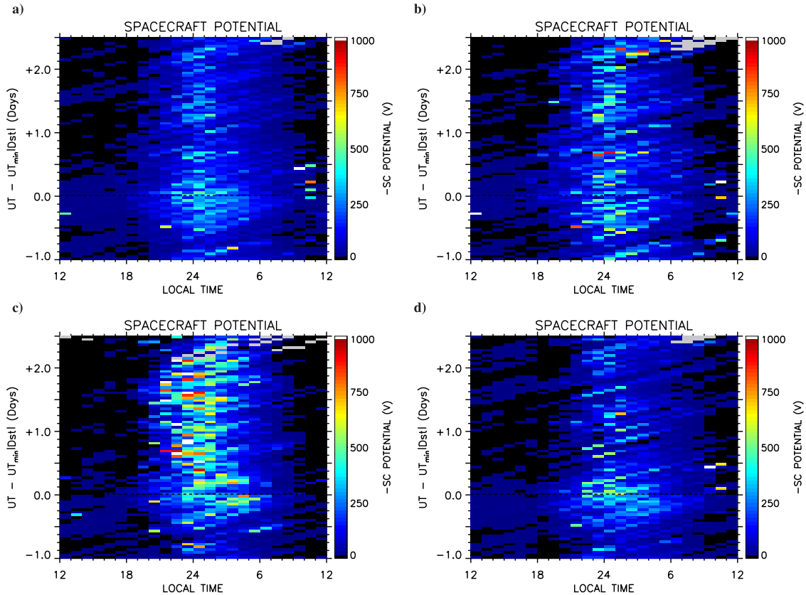
Figure 6. Same as Figure 5 except we remove all times when the spacecraft is in the Earth's shadow. The magnitude of the potential is much greater for the CIR events, compared with ICME events, and the elevated spacecraft potential lasts for a longer time.
