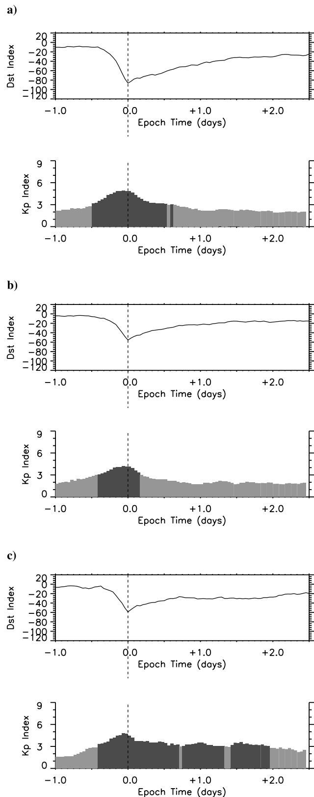
Figure 2. The mean Dst and Kp indices for the three data sets used in the study; (a) Group A - all 78 ICME events, (b) Group B - the 45 ICME events with minimum Dst > -100 , and (c) Group C - the 32 CIR events, as a function of epoch time and local time. Kp values greater than 3 are colored dark grey.
