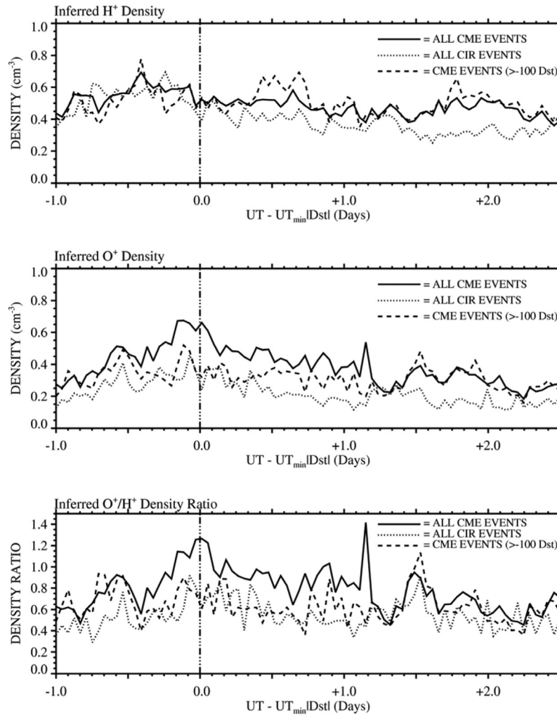
Figure 7. The averaged inferred H^+ and O^+ densities and their ratio, as a function of storm time, for Group A, Group B, and Group C events, between 2300 and 0200 LT.
