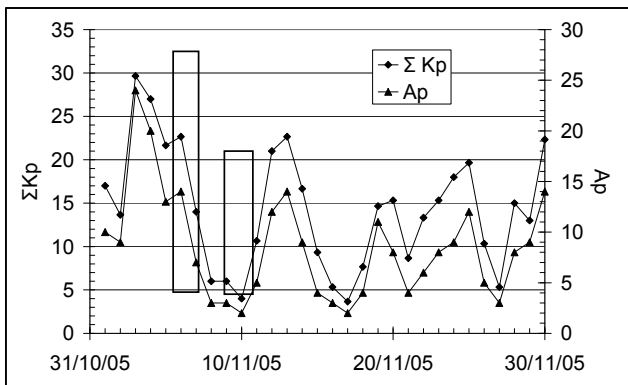
Fig. 4. k_p and A_p geomagnetic indices in November 2005
