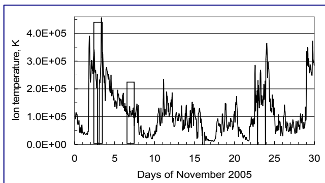
Fig. 2. Some Solar wind parameters in November 2005 (ACE data).
