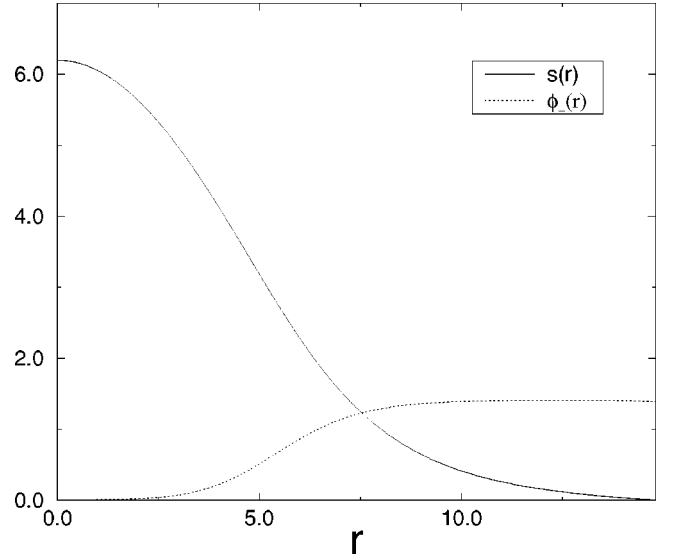
FIG. 2. Q -ball profile for \lambda=1 and g=1 .
