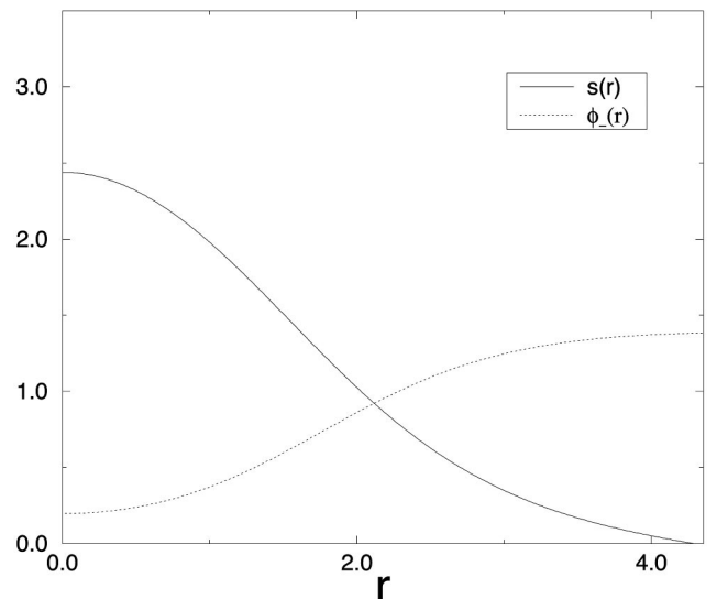
FIG. 3. Q -ball profile for \lambda = \sqrt{2} and g=1 ( F -term inflation).
