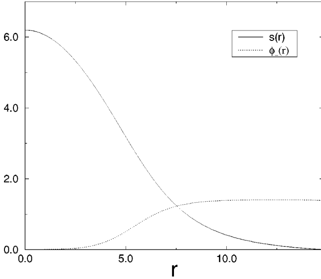
FIG. 1. Q -ball profile for \lambda=0.5 and g=1 .
