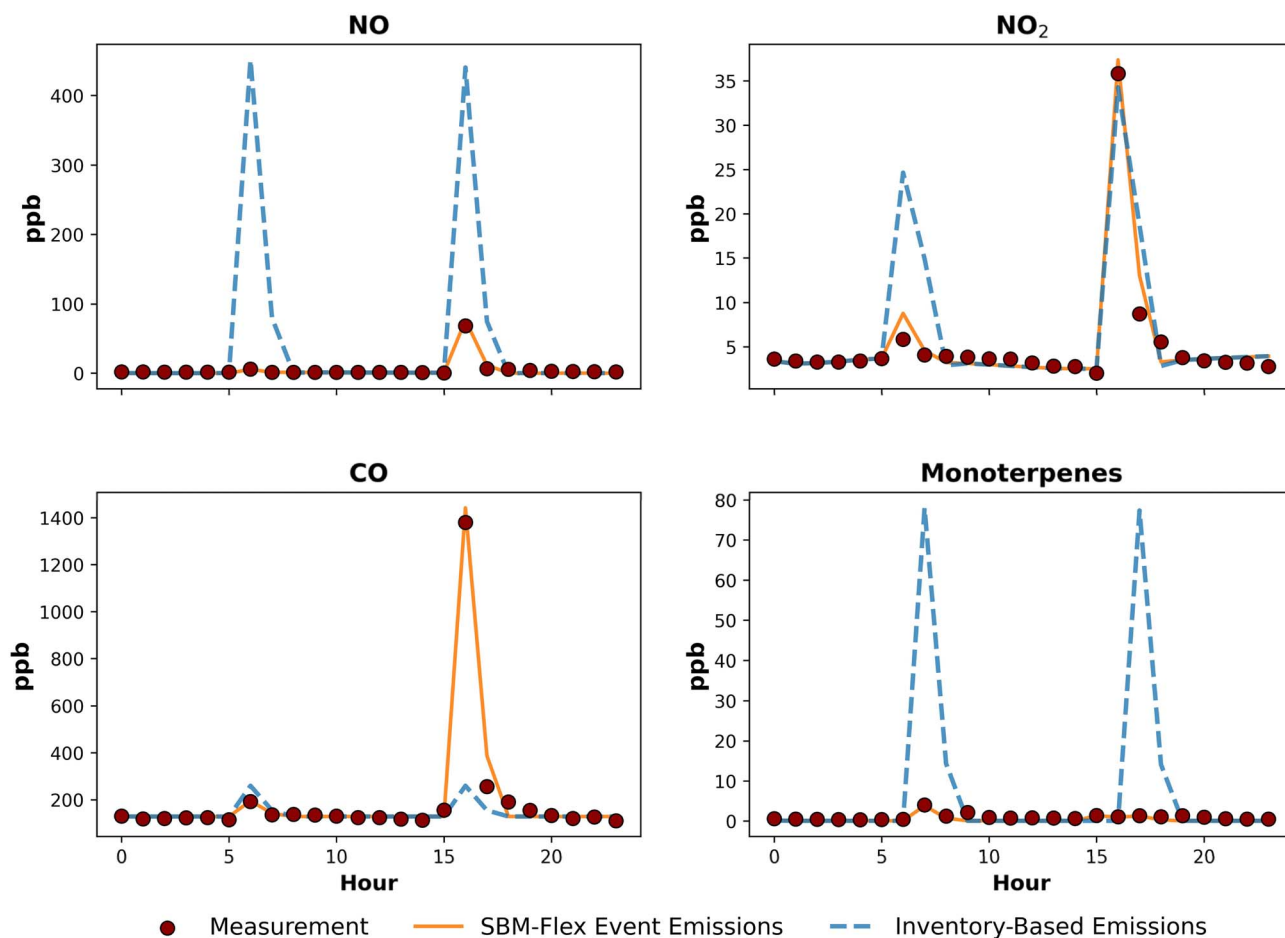
Fig. 6 Comparison of primary pollutant concentrations (NO, NO 2 , CO, and monoterpenes) simulated using the SBM-Flex Subset mechanism with event-specific emissions and inventory-based emissions against observations.
