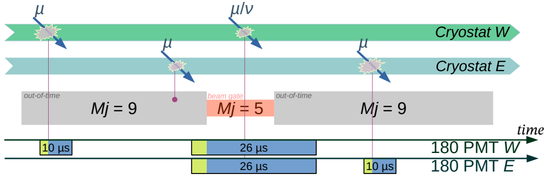
Figure 8. Schematics of the logic implemented for issuing Global and local PMT trigger primitives and of the corresponding readout of the PMT waveforms.
