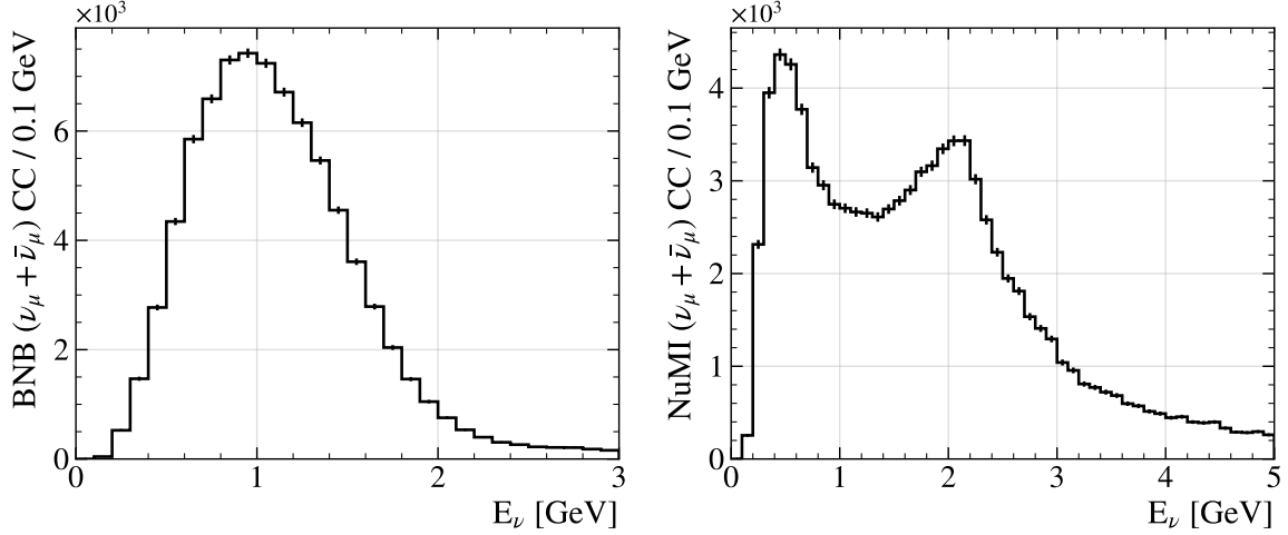
Figure 1. Charged current interaction spectra for muon neutrinos and anti-neutrinos in the active volume of the ICARUS detector, as determined in the BNB ( left ) and NuMI off-axis ( right ) beam calculations used in [1, 5] for 10^{20} POT.
