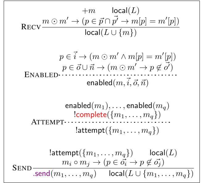
Figure 3: Operational semantics of Orpheus, as inference rules for an agent's state-transition system. Dotted line: inference within a state; solid line: transition from one state to the next. This semantics highlights the modularity of Orpheus. Rules RECV, ENABLED, and SEND are based on the BSPL semantics rendered into Jason, and implemented in our tool. The programmer is responsible only for complete to apply Rule ATTEMPT.
