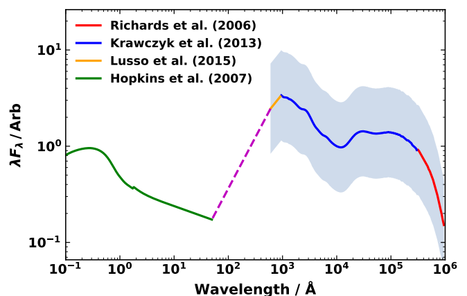
Fig. 4: The broad-band mean quasar SED introduced in Shen et al. (2020) which we assign to unobscured AGN, normalised at 1 \mu\text{m} . This SED is a combination of multiple templates from the literature: IR template of Richards et al. (2006a, red), optical/UV SED template of Krawczyk et al. (2013, blue), EUV power-law model based on the spectral index of Lusso et al. (2015, orange), which is directly connected (magenta) to the X-ray template of Hopkins et al. (2007, green). The template in this figure is a rest-frame realization of the SED with no IGM absorption, generated with the mean \alpha_{\text{ox}} of Lusso et al. (2010), \langle \alpha_{\text{ox}} \rangle = -1.37 . The blue shaded region indicates the range in possible realisations of the optical portion of the SED considering \alpha_{\text{ox}} values with the reported dispersion of 0.18.
