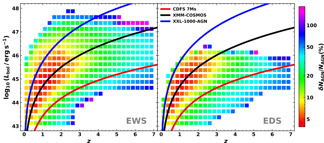
Fig. 11: Fractional uncertainty ( \delta N_{\text{AGN}}/N_{\text{AGN}} ) on the number of AGN detectable in at least one Euclid band in bins of redshift ( \Delta z = 0.25 ) and bolometric luminosity ( \Delta \log_{10}[L_{\text{bol}}/\text{erg s}^{-1}] = 0.25 ) for the EWS (left) and EDS (right). The fractional uncertainties were derived using three hundred realisations of the adopted XLF probing the \pm 1\sigma interval of each parameter given in Table 1. For reference, we plot curves corresponding to the 50% completeness flux limits of the 7 Ms exposure of the Chandra Deep Field-South (red, F_{2-7\text{keV}} = 2.5 \times 10^{-16} \text{ erg s}^{-1} \text{ cm}^{-2} ; Luo et al. 2017) and medium-depth X-ray survey XMM-COSMOS (black, F_{2-10\text{keV}} = 5.6 \times 10^{-15} \text{ erg s}^{-1} \text{ cm}^{-2} ; Cappelluti et al. 2009). We additionally show the sample limiting flux of the XXL 1000 brightest AGN sample (XXL-1000-AGN) as used in Fotopoulou et al. (2016b) for SED fitting (blue; F_{2-10\text{keV}} = 4.8 \times 10^{-14} \text{ erg s}^{-1} \text{ cm}^{-2} ; Fotopoulou et al. 2016b). The flux limits were homogenised to the 2–10 keV band assuming an X-ray power law with photon index \Gamma = 1.9 , where applicable, and converted to the bolometric domain assuming the X-ray bolometric correction of Duras et al. (2020).
