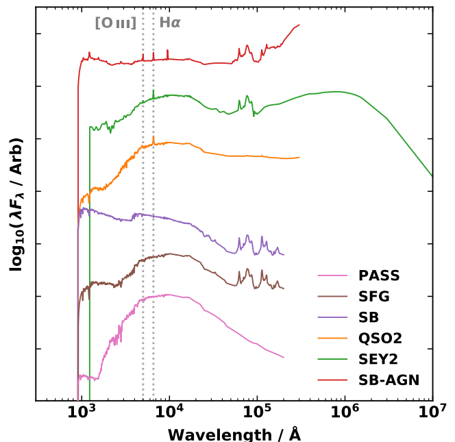
Fig. 5: Representative SEDs utilized for each obscured AGN SED class (‘PASS’: pink, ‘SFG’: brown, ‘SB’: purple, ‘QSO2’: orange, ‘SEY2’: green, ‘SB-AGN’: red) in this work. Based on the SED shapes in Fotopoulou et al. (2016b). Grey dotted lines highlight the rest-frame wavelength of the [\text{O III}]\lambda 5007 \text{ \AA} and \text{H}\alpha emission lines. Templates are assigned based on the relative probability of each template class in high- and low-luminosity groups at a given redshift.
