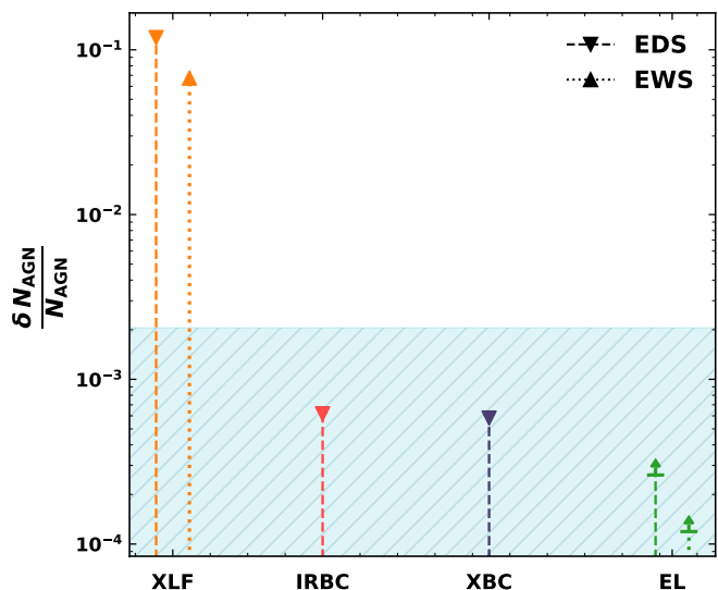
Fig. 12: Relative 1\sigma uncertainty of the number of AGN detectable in at least one Euclid band ( N_{AGN} ) for each of the quantified sources of uncertainty introduced in this work. Displayed in this plot are uncertainties introduced by the X-ray luminosity function (XLF), infrared bolometric correction dispersion (IRBC), X-ray bolometric correction dispersion (XBC) and unobscured AGN emission lines (EL) for which a lower limit was quantified using the Ly\alpha emission line and H\alpha+[N II] complex. The expected relative Poisson noise for the EDS, calculated as \sigma = \sqrt{N_{AGN}} , is indicated by the shaded blue region.
