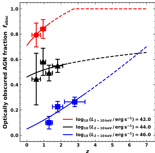
Fig. 3: Evolution of the Merloni et al. (2014) optically obscured AGN fraction as a function of redshift for different L_{2-10\text{keV}} values probed. The data points with error bars show the empirical data reproduced from Merloni et al. (2014), which was used to derive their model. The dashed lines depict extrapolation of the model.
