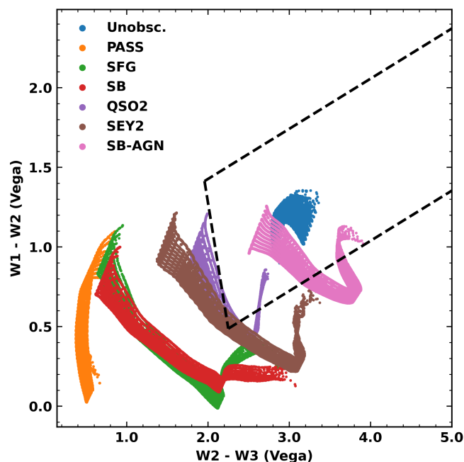
Fig. C.3: WISE three-colour selection of Mateos et al. (2012) applied to our EDS AGN. This selection uses the WISE 3.4, 4.6, and 12 \mu\text{m} bands ( W1 , W2 , and W3 respectively). We plot only AGN with S/N > 5 in at least one Euclid band and with z < 2 . Each of our AGN SED classes are plotted individually with corresponding colours identical to Fig. C.1.
