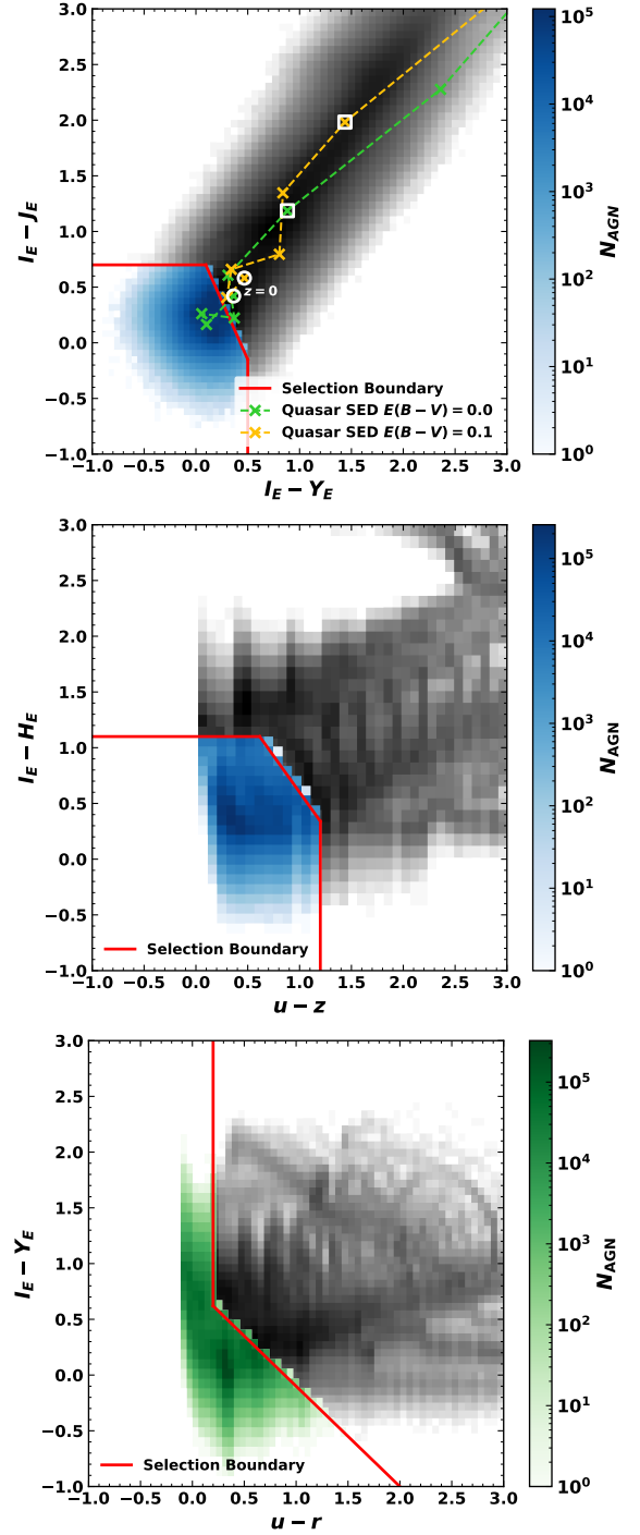
Fig. E.1: Optimal Euclid photometry AGN selection criteria derived in Euclid Collaboration: Bisigello et al. (2024) for the EWS applied to our data. We show two-dimensional density plots for AGN that are detected above the 5\sigma point-source depths in all four relevant bands. The coloured regions show the selected AGN and grey regions show non-selected AGN. Panels show selections for unobscured AGN with Euclid photometry only (top), unobscured AGN with Euclid and Rubin/LSST photometry (middle) and all AGN with Euclid and Rubin/LSST photometry (bottom). In the top panel we plot the colour-space redshift evolution of our unobscured AGN template with E(B - V) = 0 (green) and E(B - V) = 0.1 (orange) for z \in [0, 7] in steps of \delta z = 1 . White circles show the z = 0 points and white squares denote the z = 5 points. The E(B - V) = 0 green crosses in the selection region correspond to z = 1 and z = 2 .
