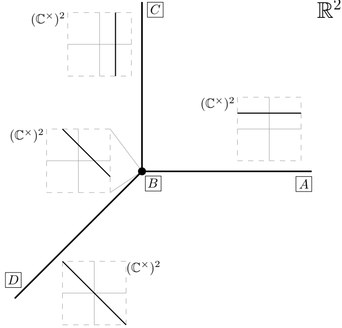
Figure 1: The fine tropical line \text{ftrop}(V^\times(P)) from Example 5.5. We view the ambient space (\mathbf{C} \times \mathbf{R})^2 as \mathbf{R}^2 with a copy of (\mathbf{C}^\times)^2 at each point. As such, \text{ftrop}(V^\times(P)) can be viewed as the usual tropical line in \mathbf{R}^2 with the subvariety of the complex torus V^\times(\text{in}_u(P)) attached at each point u \in \mathbf{R}^2 . The labels allow identification with the components given in (6) and (7).
