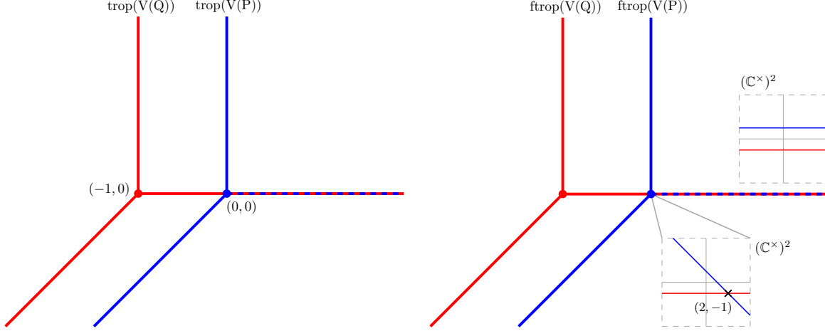
Figure 2: Left: The tropical hypersurfaces \text{trop}(V(P)) and \text{trop}(V(Q)) from Example 5.8. Note that they intersect in a 1-dim ray, but they intersect stably at a single point. Right: The fine tropical hypersurfaces \text{ftrop}(V(P)) and \text{ftrop}(V(Q)) from the same example. These do intersect transversally, and so they intersect at a single point.
