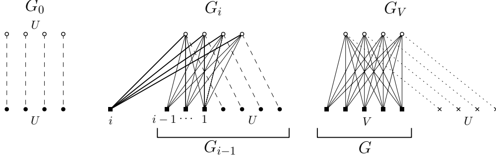
Figure 12: The inductive construction of graphs corresponding to principal extension from Lemma B.3.
