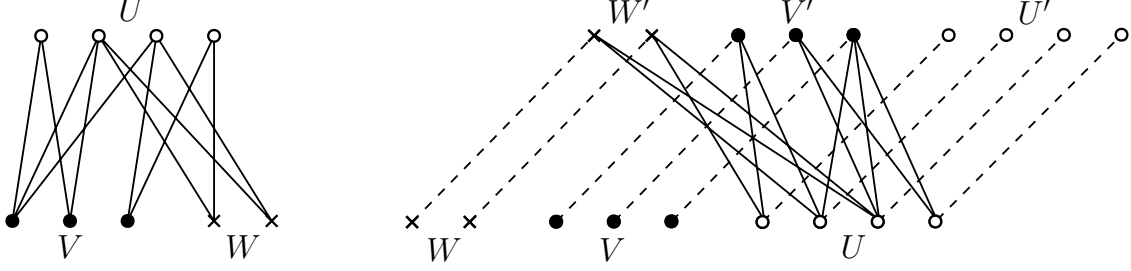
Figure 7: Construction of R-minor representation for f^* .
