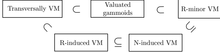
Figure 4: The inclusion relationship between classes of valuated matroids.
