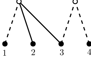
Figure 2: The bipartite graph realising the transversally valued matroid from Example 2.4. The dashed edges have weight zero and the solid edges have weight one.
