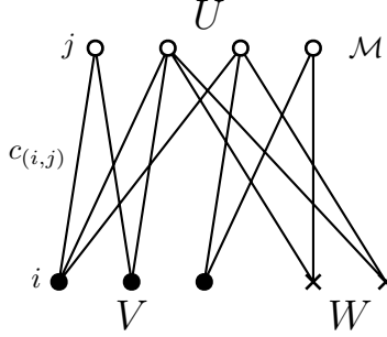
Figure 1: A bipartite graph G = (V \cup W, U; E) with edge weights c \in \mathbb{R}^E and matroid \mathcal{M} on vertex set U . This gives rise to an R-minor valuated matroid on V , as described in Definition 1.1.
