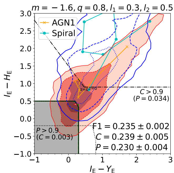
Fig. 3. Best selection (type A) criterion for AGN1 in the EDS using only Euclid filters (shaded grey area). The shaded red areas correspond to the colour distribution of AGN1, while the blue lines are the contour levels of the remaining galaxies. Levels correspond to 68%, 95%, and 99.7% of the distribution. We also present example SED tracks for one AGN1 (yellow crosses) and one spiral galaxy (cyan circles) from z = 0 to z = 6 , with steps of \Delta z = 1 . As an indication of how strict the best selection is, the two dashed green lines, which almost completely overlap with the black one, show the extent of all the best selection criteria derived with the bootstrap approach. The dotted black line and the dash-dotted black line correspond to the best selection with P > 0.9 and C > 0.9 , respectively.
