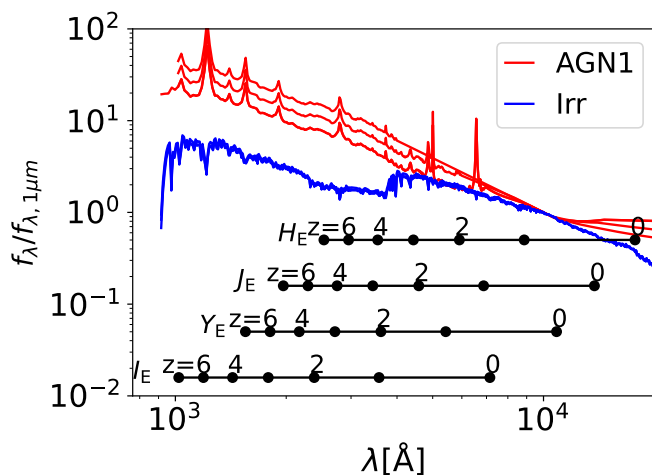
Fig. 4. SEDs of AGN1 (solid red lines) and dwarf irregulars (solid blue line), normalised at 1 \mu\text{m} . We also report the rest-frame wavelength observed by the Euclid filters at different redshifts (black circles).
