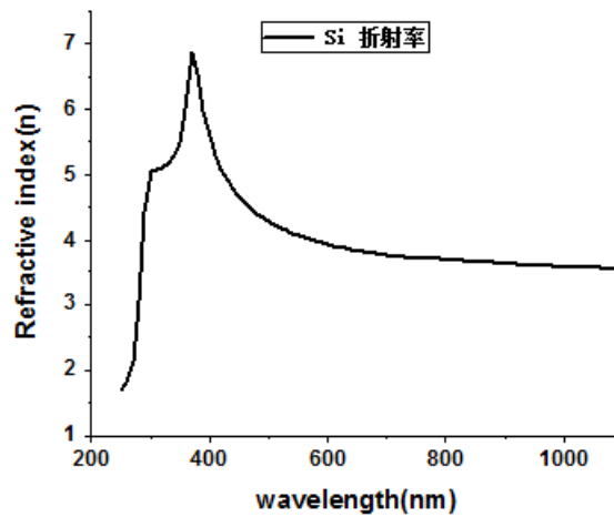
Figure 4 Curve of the refractive index of silicon dependence on wavelength
