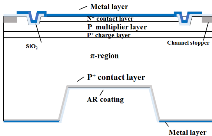
Figure 6 Broadband Si APD device structure
