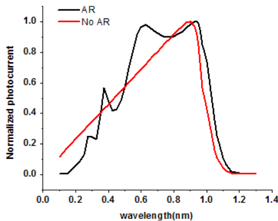
Figure 9 the Spectrum of Si APD(a)without antireflection coating (b)with antireflection coating
