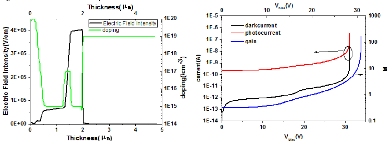
图 3 紫外增强 Si APD 的 (a) 电场分布 (b) IV 曲线及倍增曲线 Figure 3 Ultraviolet Enhanced Si APD (a) Electric Field Distribution (b) IV Curve and Multiplication Curve
