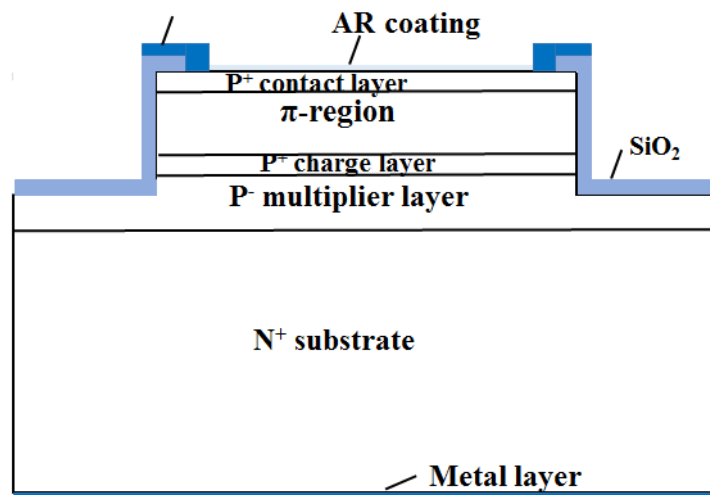
图 2 Si APD 紫外吸收器件结构图 Figure 2 Si APD ultraviolet absorption device Structure
