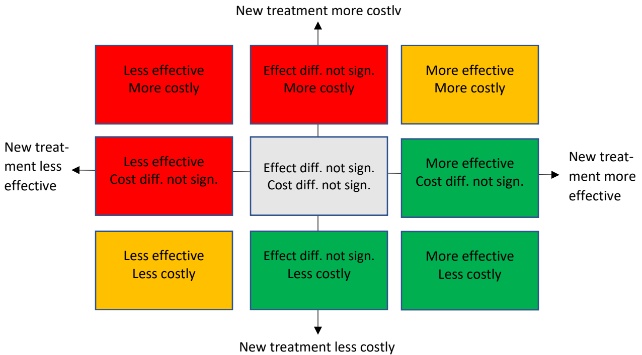
Figure 2: Generic cost-effectiveness plane
