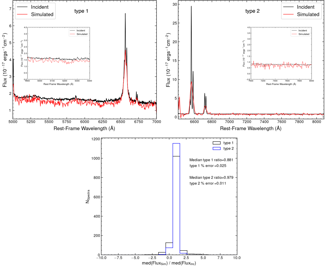
Fig. F.1. Top row: Example of a comparison between the incident (black) and simulated (red) spectra for a type 1 ( left ) and a type 2 ( right ) AGN around the H\alpha region. The inset plot is a zoom-in of a continuum (emission line free) region. Bottom row: distribution of the ratios of the median flux value (i.e., the median of the observed flux of the total spectrum) of the incident and simulated data for both type 1 (black) and type 2 (blue) AGN. The median values for the two distributions are also reported. The percentage error on the distributions of the spectrum flux median values are computed as 1.253 \sigma / \sqrt{N} , where \sigma and N represent the standard dispersion of the distribution and the number of objects, respectively.
