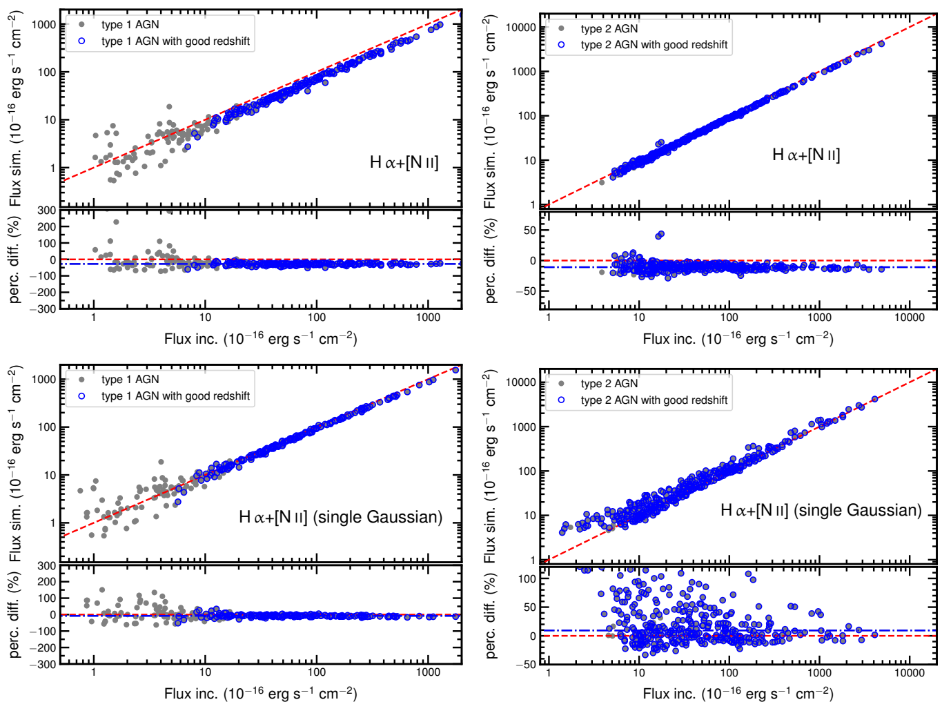
Fig. 11. Comparison of the H\alpha + [N\text{II}] flux measurement between the simulated and the incident spectra for the type 1 ( left ) and type 2 ( right ) AGN samples. Sources with a spectroscopic redshift measured from the simulated spectra and flagged as ‘good’ (see Sect. 5 for details) are marked with blue symbols. The bottom panel in each plot shows the percentage luminosity difference defined as \Delta F/F = (F_{H\alpha, \text{sim}} - F_{H\alpha, \text{inc}})/F_{H\alpha, \text{inc}} . The one-to-one flux relation is shown with a red dashed line, which is set to zero in the bottom panel. The dot-dashed blue line in the bottom panel represents the 50 th percentile of the \Delta F/F distribution. Top row : Simulated data: best fit flux obtained from the integration of a single broad component used to model the H\alpha + [N\text{II}] complex. Incident: Best fit flux obtained from the summation of the individual components used to model the H\alpha + [N\text{II}] complex for incident spectra (i.e., broad and narrow component for the H\alpha , [N\text{II}]\lambda\lambda 6549, 6583 ). Bottom row : the best fit flux of the H\alpha + [N\text{II}] complex is obtained from the integration of a single broad component for both simulated and incident data.
