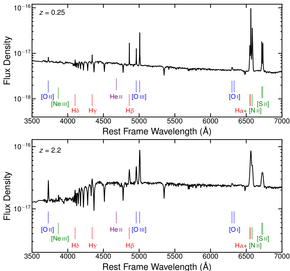
Fig. 6. Examples of obscured type 2 AGN incident spectra (flux density values are in units of \text{erg s}^{-1} \text{cm}^{-2} \text{Å}^{-1} ) at optical wavelengths, from 3500 Å to 7000 Å. Top panel: a z = 0.25 type 2 AGN with a bolometric luminosity \log_{10}(L_{\text{bol}}/\text{erg s}^{-1}) of 43.9, hosted in a galaxy with a stellar mass M_{\star} of 10^{9.2} M_{\odot} and SFR of 10^{0.9} M_{\odot} \text{yr}^{-1} . Bottom panel: a massive ( M_{\star} = 10^{11.8} M_{\odot} ) galaxy at z = 2.2 with intense star-formation (SFR = 10^{2.6} M_{\odot} \text{yr}^{-1} ) hosting an AGN with \log_{10}(L_{\text{bol}}/\text{erg s}^{-1}) = 45.2 . The main emission lines are marked.
