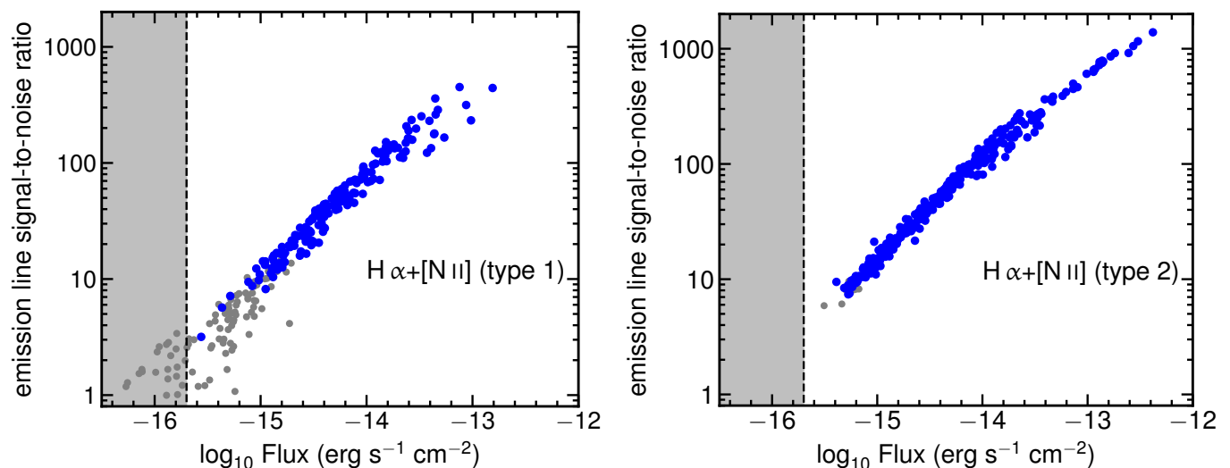
Fig. 12. Emission line signal-to-noise ratio as a function of the total integrated flux for H\alpha+[N\text{ II}] observed in the simulated spectra in type 1 ( left ) and type 2 ( right ) AGN. The dashed line marks the H\alpha flux limit of the Euclid survey of 2 \times 10^{-16} \text{ erg s}^{-1} \text{ cm}^{-2} . Symbols are as in Fig. 11.
