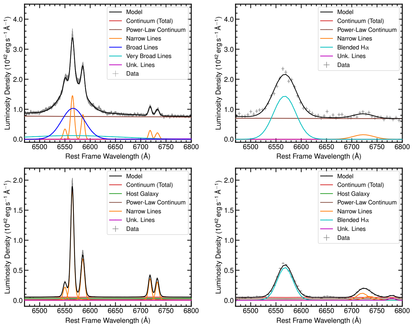
Fig. 9. Example showing type 1 ( top row ) and type 2 ( bottom row ) AGN H\alpha complex of incident ( left ) and Euclid -like simulated spectra ( right ). The sources shown in this plot have redshifts z = 1.7 (type 1) and z = 1.2 (type 2).
