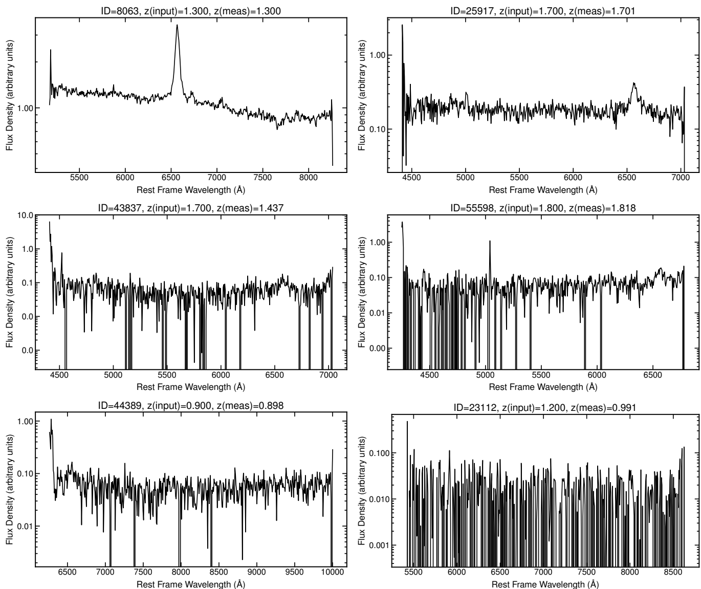
Fig. A.1. Example of Euclid -like simulated spectra for type 1 AGN in the redshift interval 0.89 \leq z \leq 1.83 , thus where the H\alpha + [N II] complex is within the spectral coverage of the red grism. Spectra are shown at different SNR and noise levels (medium/high on the left and low on the right) for the good (top row), false (mid row), and lost (bottom row) redshift classes (see Sect. 5).
