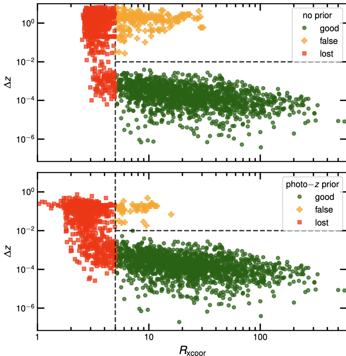
Fig. 8. Redshift uncertainty \Delta z (defined as |z_{\text{out}} - z_{\text{in}}| ) for the total sample of 2496 AGN as a function of the parameter R_{\text{xccor}} (that is related to the shape of the correlation peak, and is inversely proportional to the redshift measurement uncertainty) when using no prior ( upper panel ) and photometric redshift prior ( lower panel ). Different colours refer to different classifications of the redshift estimates (see Sect. 5 for more details).
