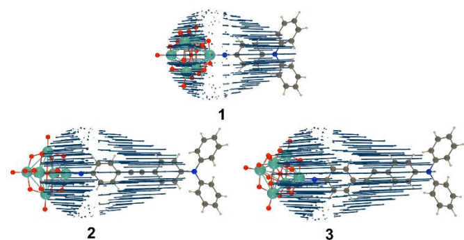
Fig. 4 Unit sphere representations (USRs) of the \beta tensor ( \lambda = 1200 nm) of compounds 1 to 3 calculated at the IEFFPCM (solvent = acetonitrile) TDDFT/ \omega B97X-D/6-311G(d)/LanL2TZ level of theory. (USR factor of 0.0001).
